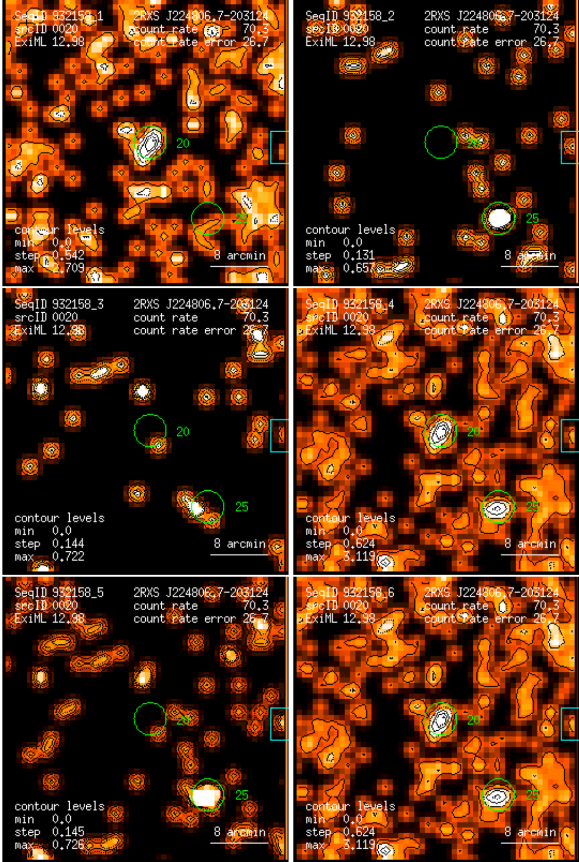
Figure 20: RASS 932158: detection 0020: band rate images, Gaussian filter: (1) PSPC channels 11 – 41, (2) 52 – 90, (3) 91 – 201, (4) 11 – 235, (5) 52 – 201, (6) 11 – 201. Broad band rates in counts/ks. Band rate contour levels in counts/ks/arcmin 2 .
