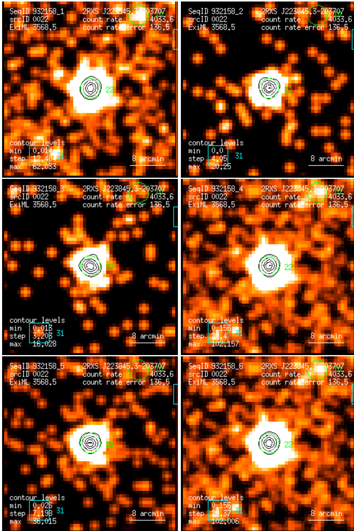
Figure 22: RASS 932158: detection 0022: band rate images, Gaussian filter: (1) PSPC channels 11 – 41, (2) 52 – 90, (3) 91 – 201, (4) 11 – 235, (5) 52 – 201, (6) 11 – 201. Broad band rates in counts/ks. Band rate contour levels in counts/ks/arcmin 2 .
