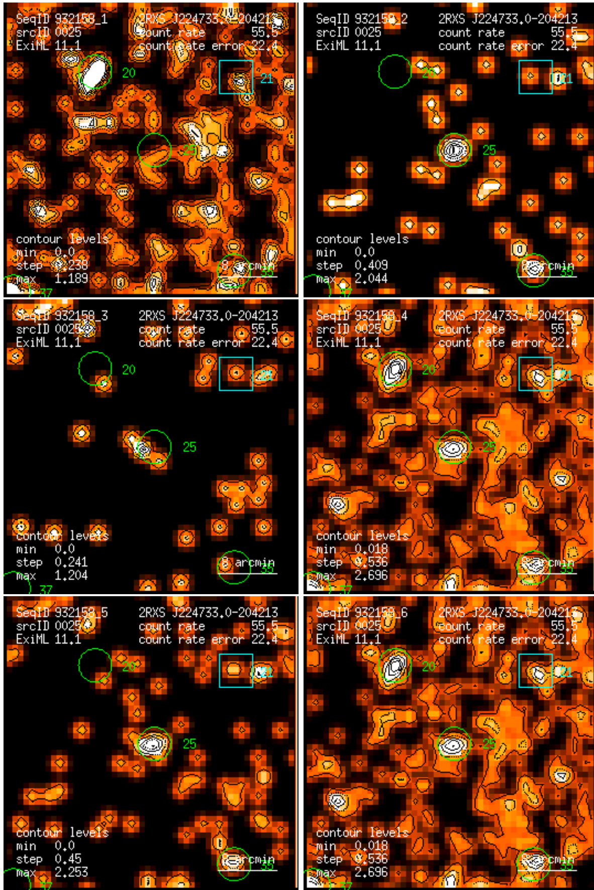
Figure 25: RASS 932158: detection 0025: band rate images, Gaussian filter: (1) PSPC channels 11 – 41, (2) 52 – 90, (3) 91 – 201, (4) 11 – 235, (5) 52 – 201, (6) 11 – 201. Broad band rates in counts/ks. Band rate contour levels in counts/ks/arcmin 2 .
