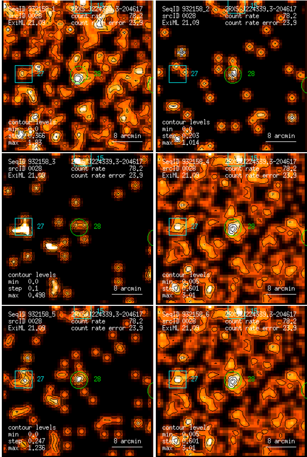
Figure 28: RASS 932158: detection 0028: band rate images, Gaussian filter: (1) PSPC channels 11 – 41, (2) 52 – 90, (3) 91 – 201, (4) 11 – 235, (5) 52 – 201, (6) 11 – 201. Broad band rates in counts/ks. Band rate contour levels in counts/ks/arcmin 2 .
