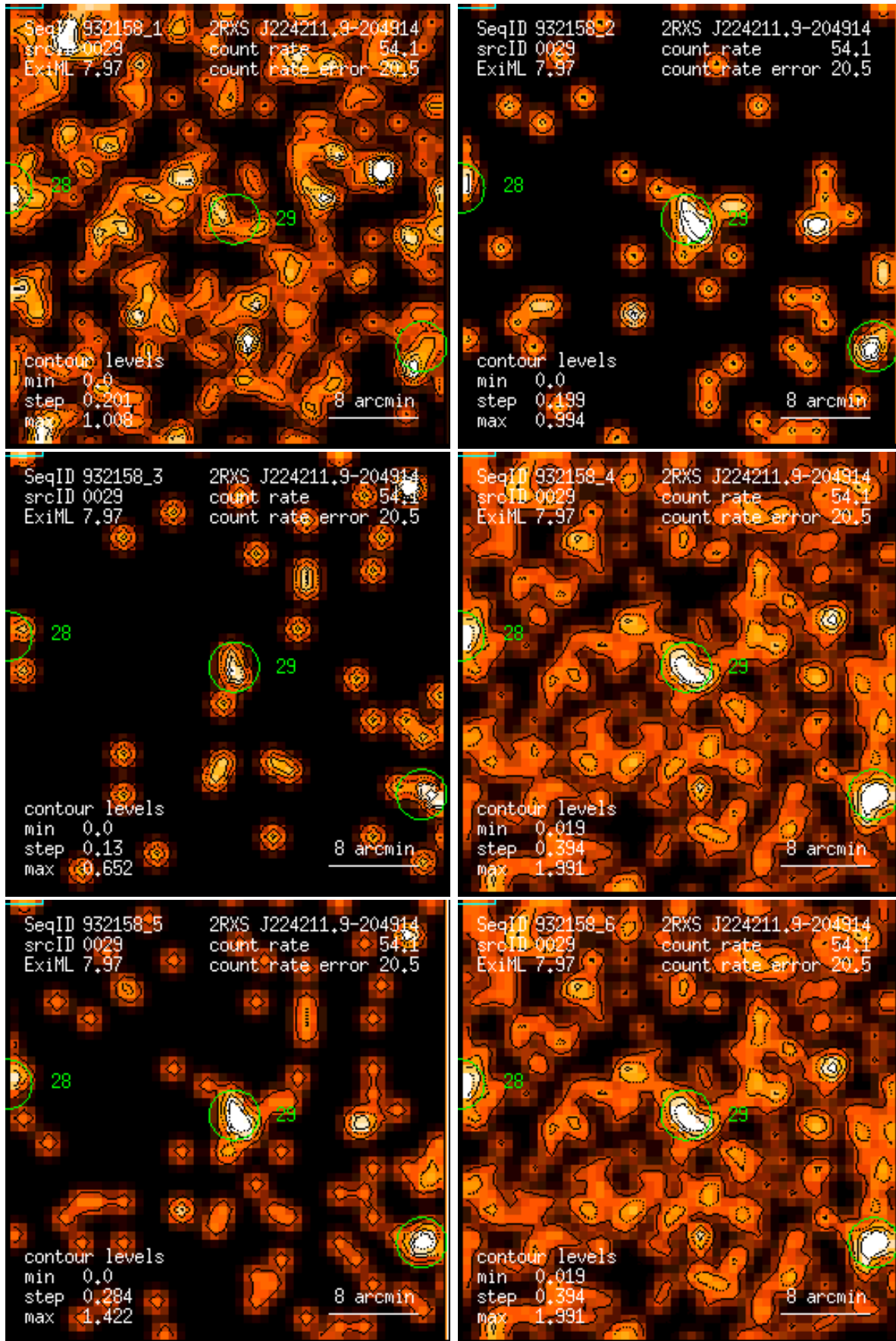
Figure 29: RASS 932158: detection 0029: band rate images, Gaussian filter: (1) PSPC channels 11 – 41, (2) 52 – 90, (3) 91 – 201, (4) 11 – 235, (5) 52 – 201, (6) 11 – 201. Broad band rates in counts/ks. Band rate contour levels in counts/ks/arcmin 2 .
