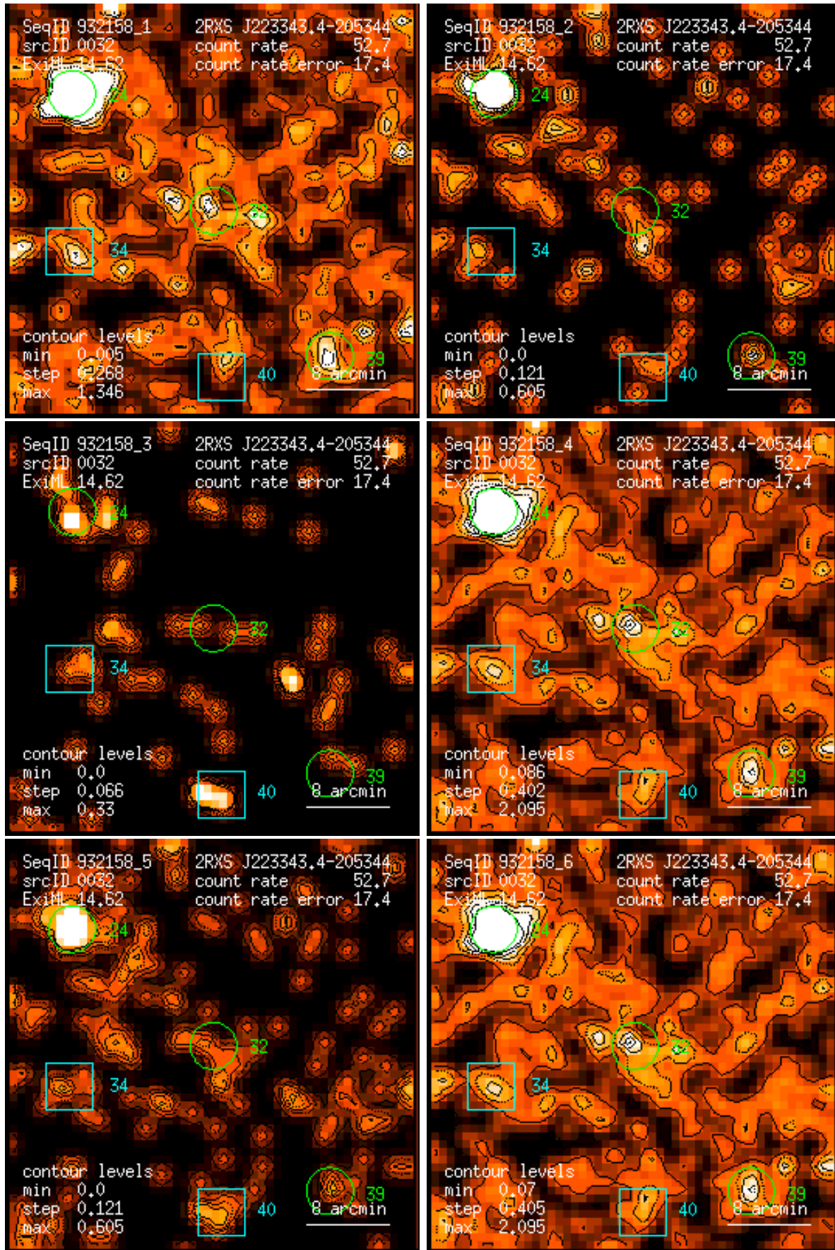
Figure 32: RASS 932158: detection 0032: band rate images, Gaussian filter: (1) PSPC channels 11 – 41, (2) 52 – 90, (3) 91 – 201, (4) 11 – 235, (5) 52 – 201, (6) 11 – 201. Broad band rates in counts/ks. Band rate contour levels in counts/ks/arcmin 2 .
