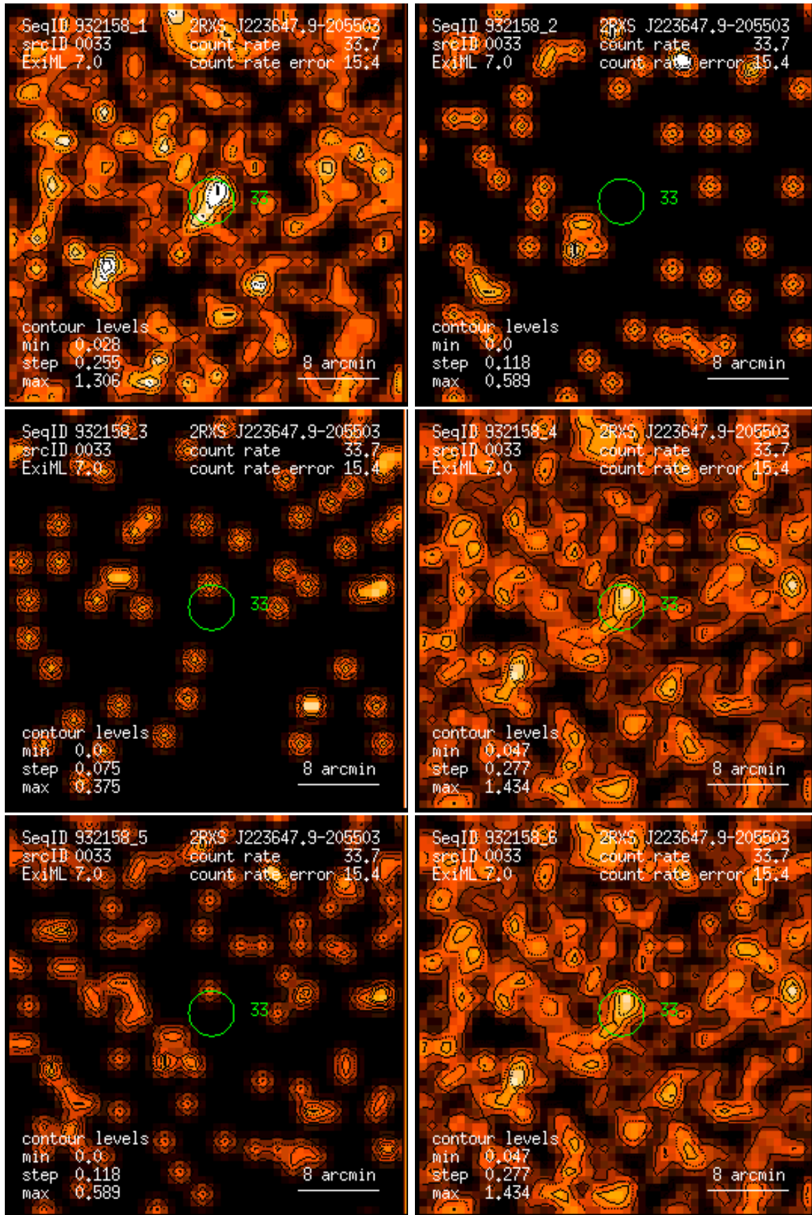
Figure 33: RASS 932158: detection 0033: band rate images, Gaussian filter: (1) PSPC channels 11 – 41, (2) 52 – 90, (3) 91 – 201, (4) 11 – 235, (5) 52 – 201, (6) 11 – 201. Broad band rates in counts/ks. Band rate contour levels in counts/ks/arcmin 2 .
