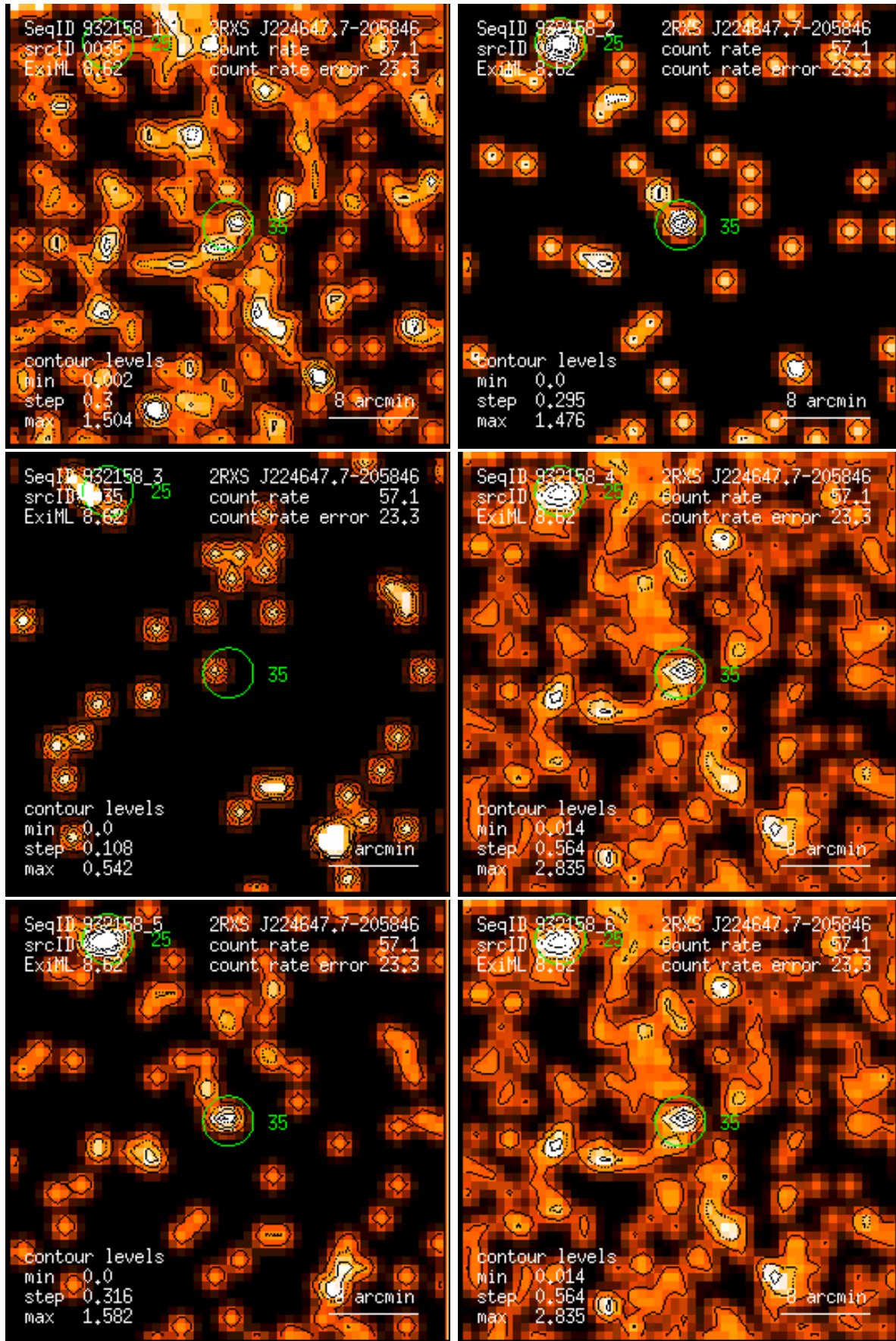
Figure 35: RASS 932158: detection 0035: band rate images, Gaussian filter: (1) PSPC channels 11 – 41, (2) 52 – 90, (3) 91 – 201, (4) 11 – 235, (5) 52 – 201, (6) 11 – 201. Broad band rates in counts/ks. Band rate contour levels in counts/ks/arcmin 2 .
