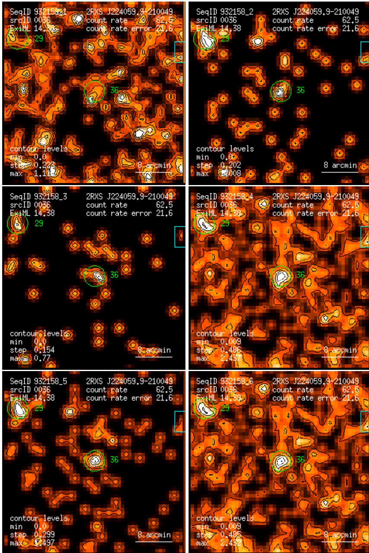
Figure 36: RASS 932158: detection 0036: band rate images, Gaussian filter: (1) PSPC channels 11 – 41, (2) 52 – 90, (3) 91 – 201, (4) 11 – 235, (5) 52 – 201, (6) 11 – 201. Broad band rates in counts/ks. Band rate contour levels in counts/ks/arcmin 2 .
