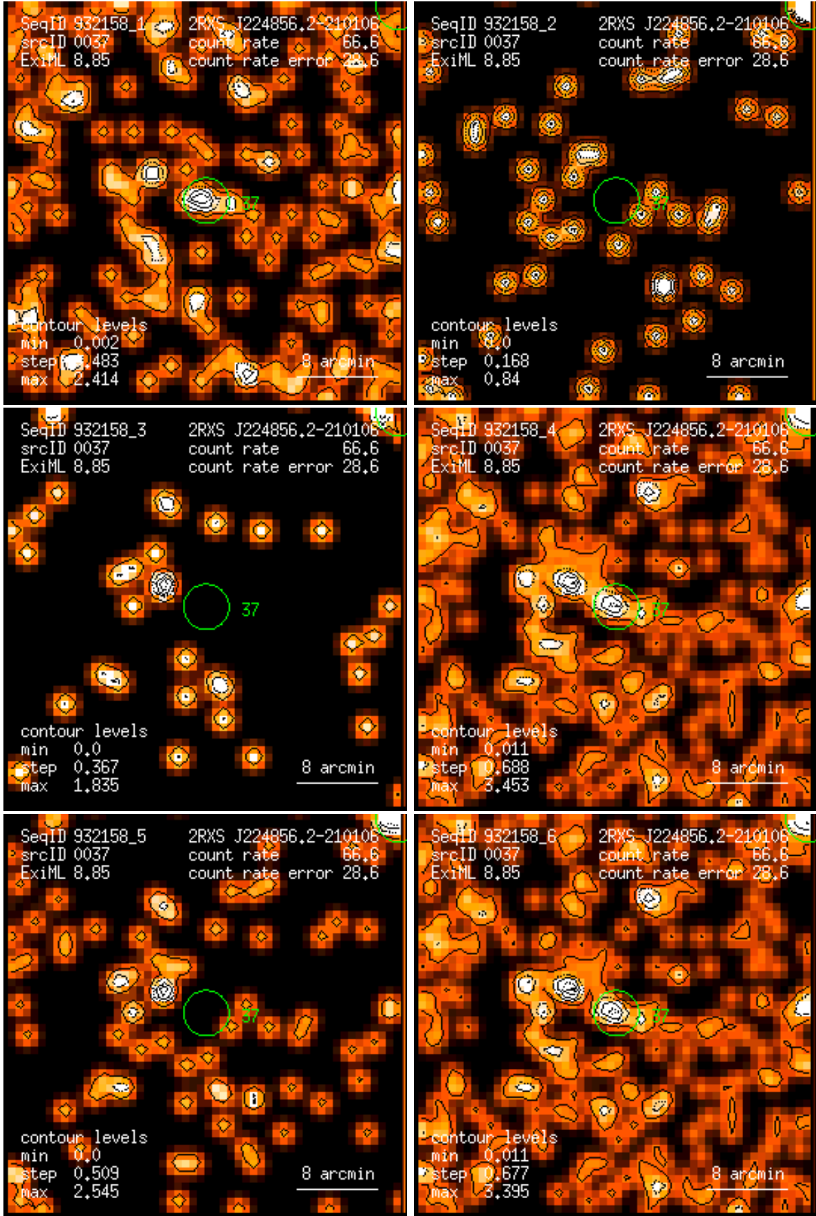
Figure 37: RASS 932158: detection 0037: band rate images, Gaussian filter: (1) PSPC channels 11 – 41, (2) 52 – 90, (3) 91 – 201, (4) 11 – 235, (5) 52 – 201, (6) 11 – 201. Broad band rates in counts/ks. Band rate contour levels in counts/ks/arcmin 2 .
