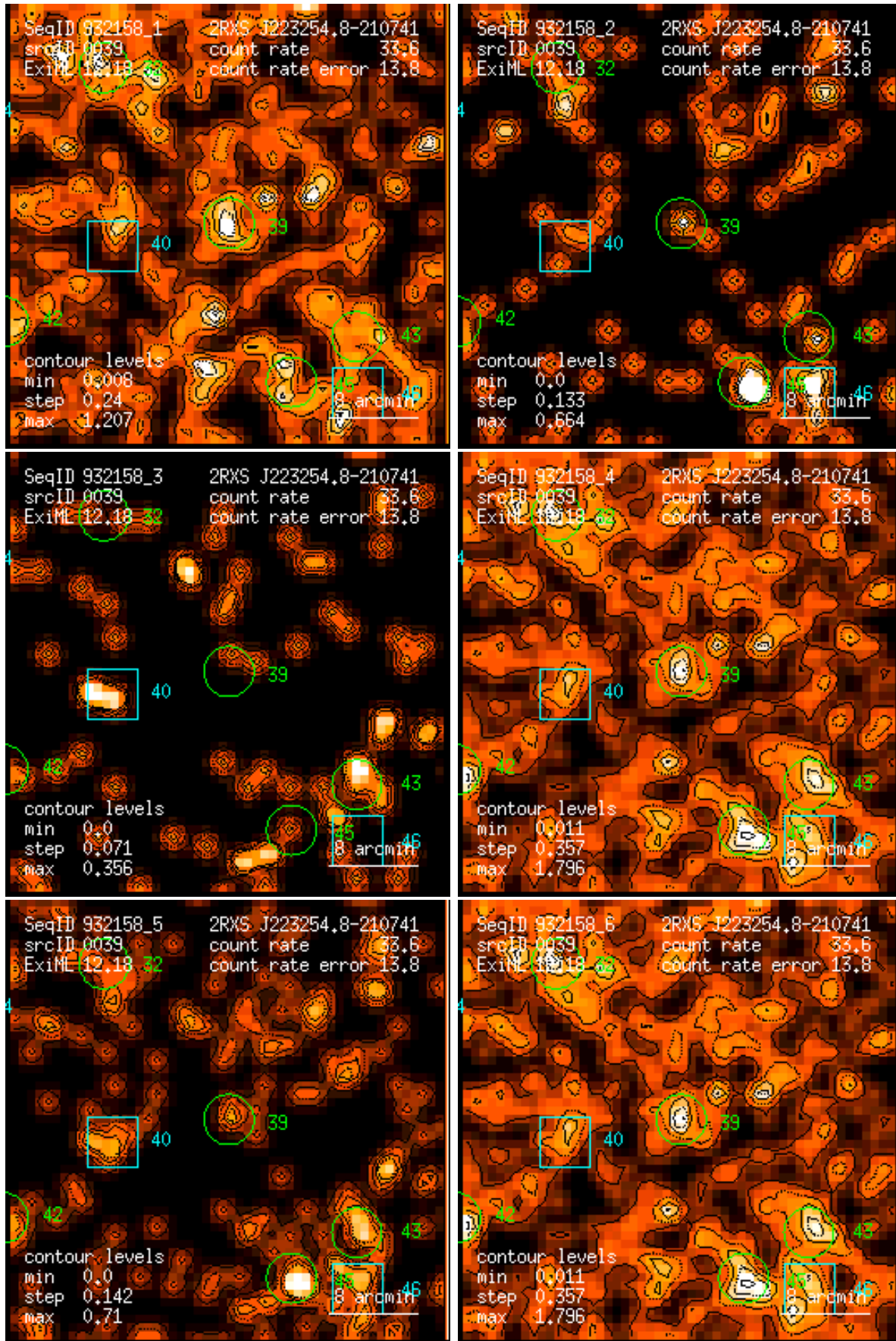
Figure 39: RASS 932158: detection 0039: band rate images, Gaussian filter: (1) PSPC channels 11 – 41, (2) 52 – 90, (3) 91 – 201, (4) 11 – 235, (5) 52 – 201, (6) 11 – 201. Broad band rates in counts/ks. Band rate contour levels in counts/ks/arcmin 2 .
