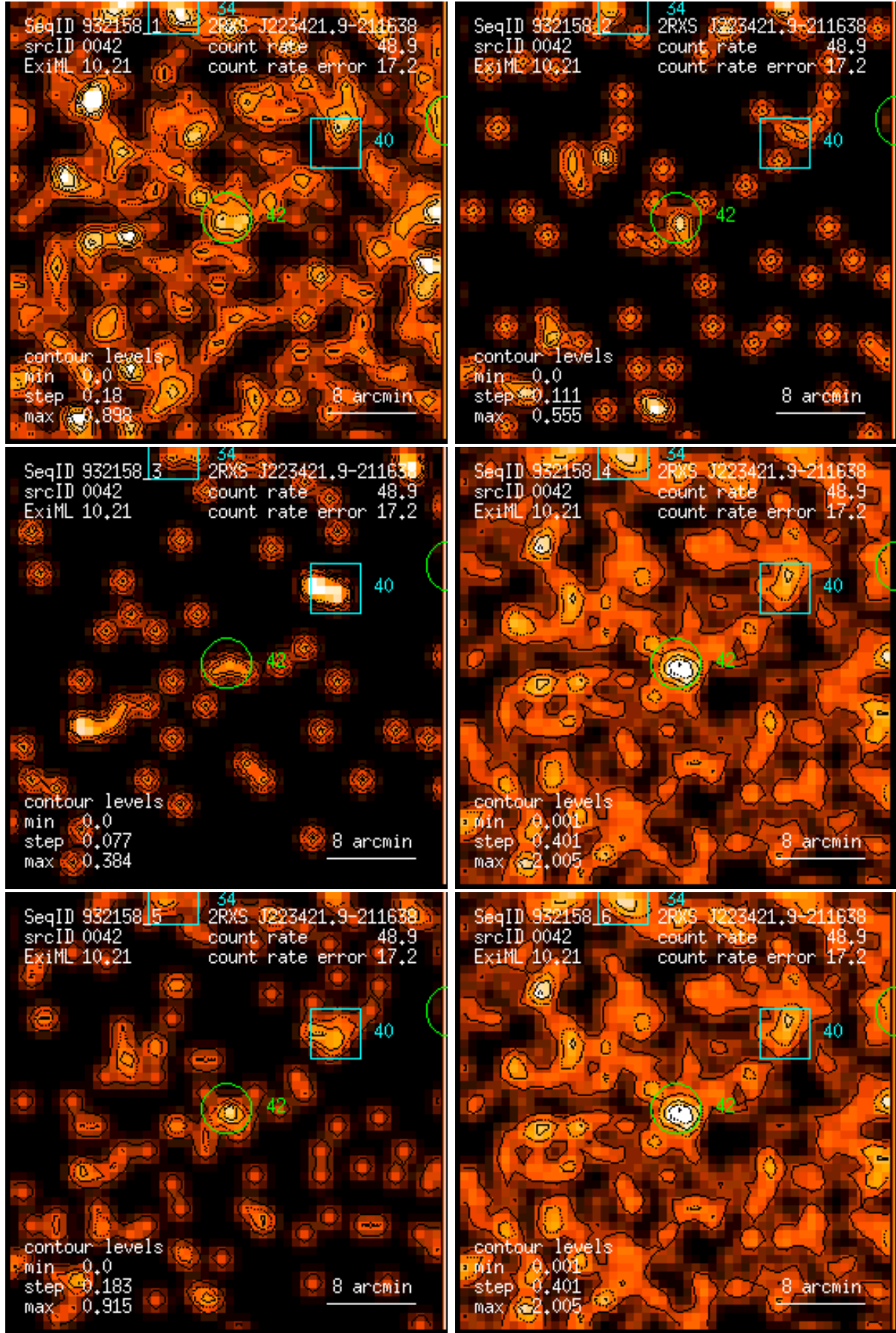
Figure 42: RASS 932158: detection 0042: band rate images, Gaussian filter: (1) PSPC channels 11 – 41, (2) 52 – 90, (3) 91 – 201, (4) 11 – 235, (5) 52 – 201, (6) 11 – 201. Broad band rates in counts/ks. Band rate contour levels in counts/ks/arcmin 2 .
