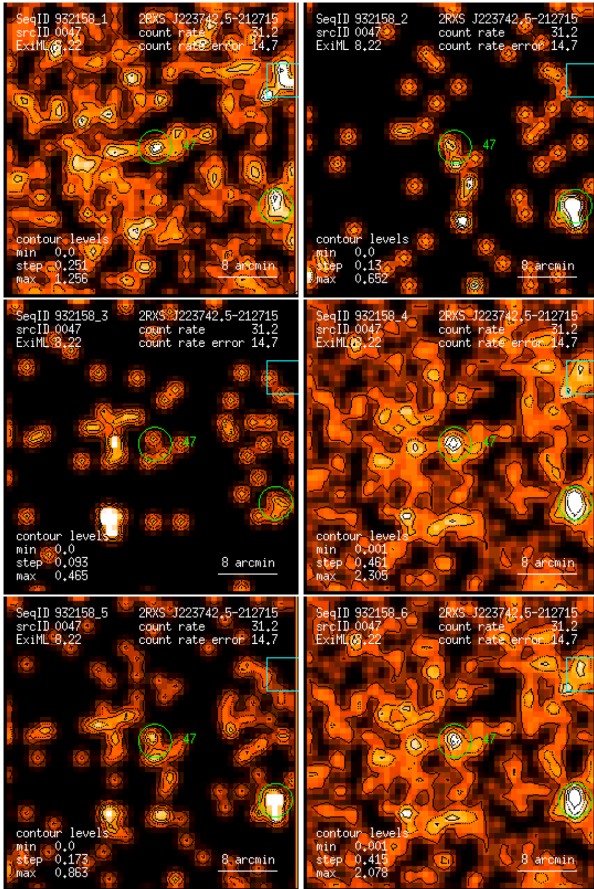
Figure 47: RASS 932158: detection 0047: band rate images, Gaussian filter: (1) PSPC channels 11 – 41, (2) 52 – 90, (3) 91 – 201, (4) 11 – 235, (5) 52 – 201, (6) 11 – 201. Broad band rates in counts/ks. Band rate contour levels in counts/ks/arcmin 2 .
