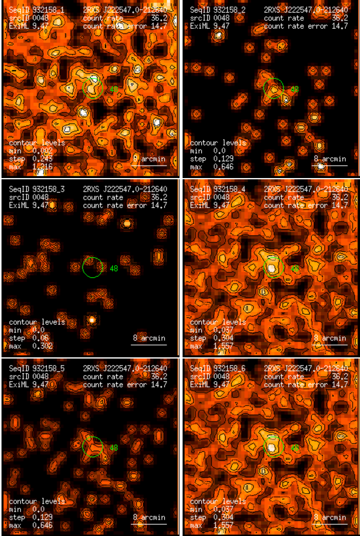
Figure 48: RASS 932158: detection 0048: band rate images, Gaussian filter: (1) PSPC channels 11 – 41, (2) 52 – 90, (3) 91 – 201, (4) 11 – 235, (5) 52 – 201, (6) 11 – 201. Broad band rates in counts/ks. Band rate contour levels in counts/ks/arcmin 2 .
