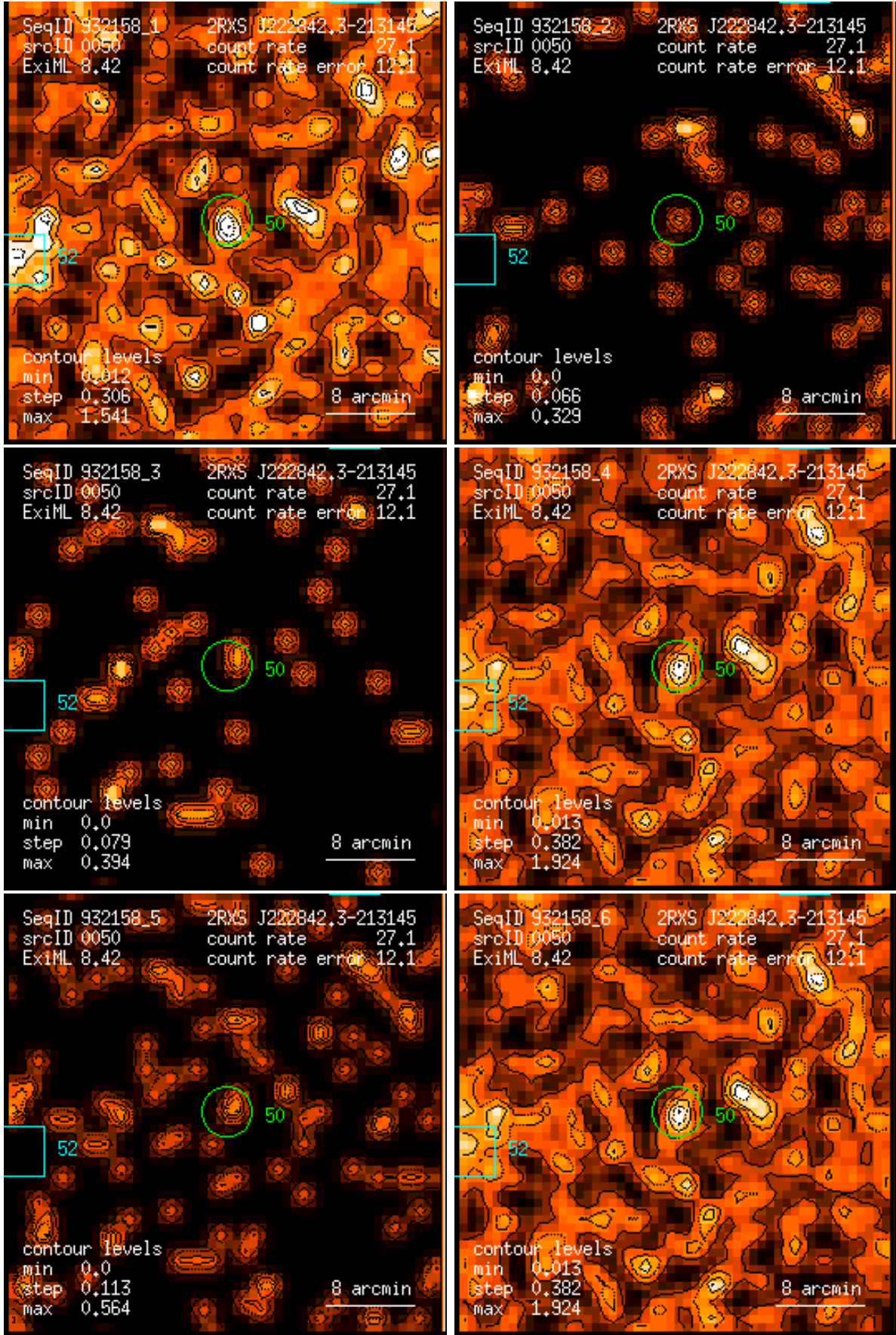
Figure 50: RASS 932158: detection 0050: band rate images, Gaussian filter: (1) PSPC channels 11 – 41, (2) 52 – 90, (3) 91 – 201, (4) 11 – 235, (5) 52 – 201, (6) 11 – 201. Broad band rates in counts/ks. Band rate contour levels in counts/ks/arcmin 2 .
