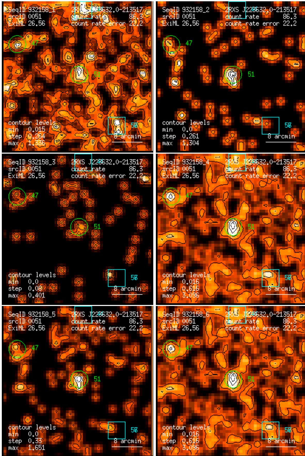
Figure 51: RASS 932158: detection 0051: band rate images, Gaussian filter: (1) PSPC channels 11 – 41, (2) 52 – 90, (3) 91 – 201, (4) 11 – 235, (5) 52 – 201, (6) 11 – 201. Broad band rates in counts/ks. Band rate contour levels in counts/ks/arcmin 2 .
