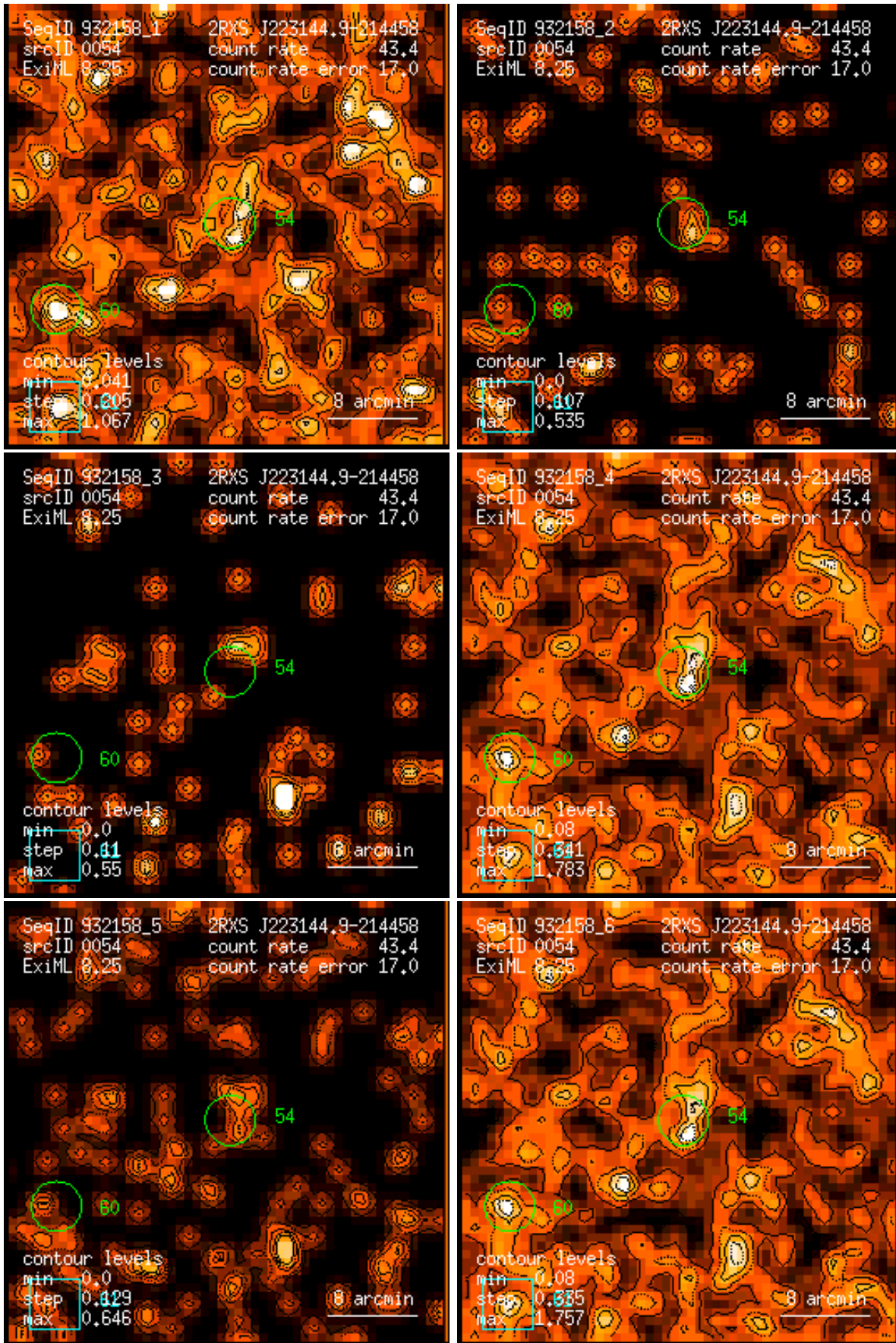
Figure 54: RASS 932158: detection 0054: band rate images, Gaussian filter: (1) PSPC channels 11 – 41, (2) 52 – 90, (3) 91 – 201, (4) 11 – 235, (5) 52 – 201, (6) 11 – 201. Broad band rates in counts/ks. Band rate contour levels in counts/ks/arcmin 2 .
