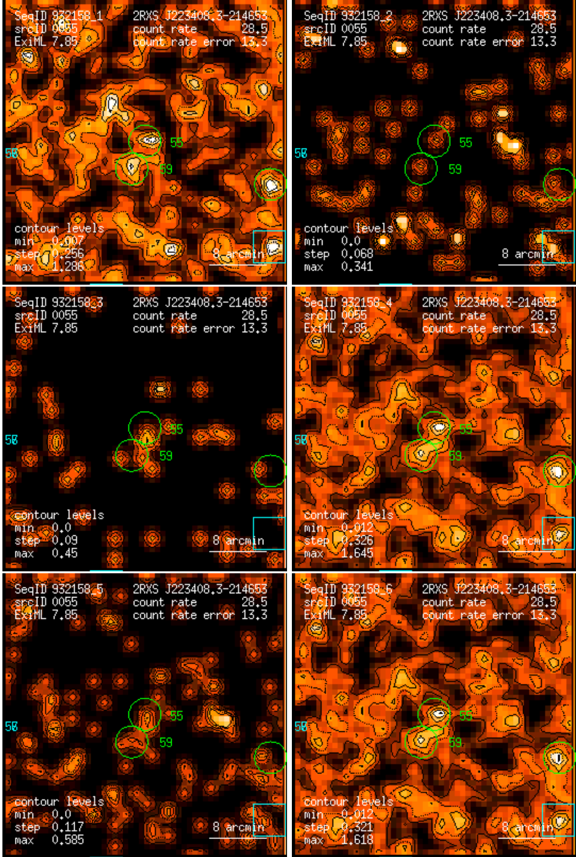
Figure 55: RASS 932158: detection 0055: band rate images, Gaussian filter: (1) PSPC channels 11 – 41, (2) 52 – 90, (3) 91 – 201, (4) 11 – 235, (5) 52 – 201, (6) 11 – 201. Broad band rates in counts/ks. Band rate contour levels in counts/ks/arcmin 2 .
