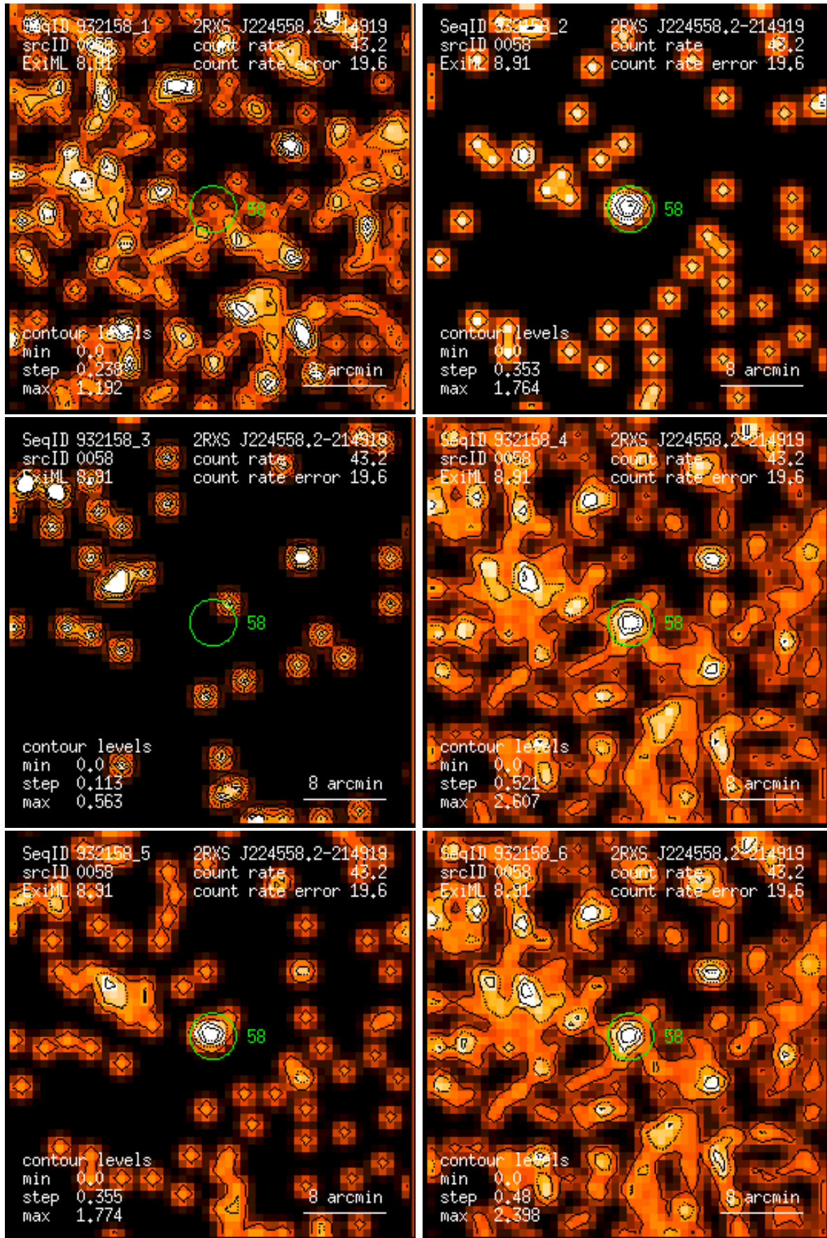
Figure 58: RASS 932158: detection 0058: band rate images, Gaussian filter: (1) PSPC channels 11 – 41, (2) 52 – 90, (3) 91 – 201, (4) 11 – 235, (5) 52 – 201, (6) 11 – 201. Broad band rates in counts/ks. Band rate contour levels in counts/ks/arcmin 2 .
