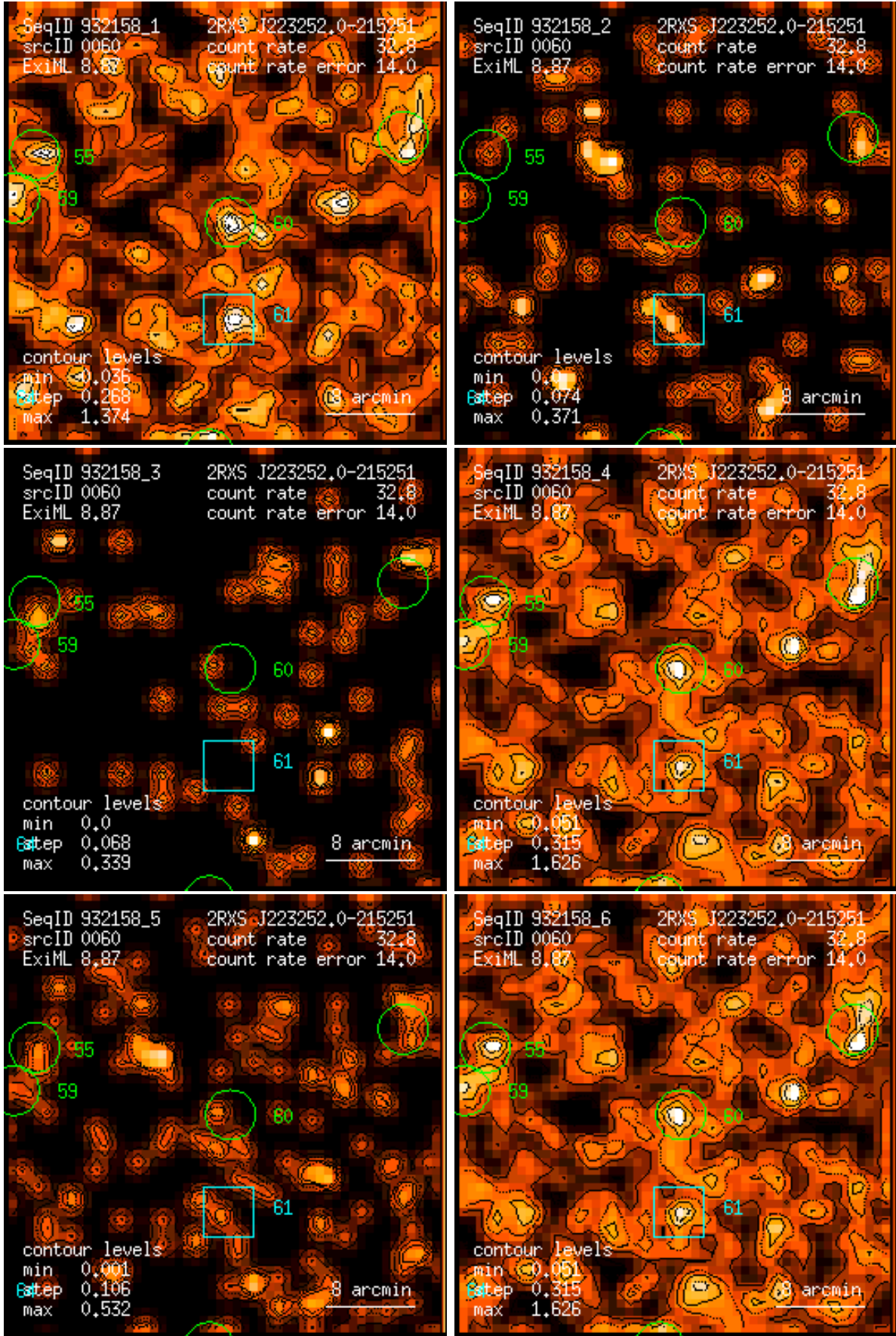
Figure 60: RASS 932158: detection 0060: band rate images, Gaussian filter: (1) PSPC channels 11 – 41, (2) 52 – 90, (3) 91 – 201, (4) 11 – 235, (5) 52 – 201, (6) 11 – 201. Broad band rates in counts/ks. Band rate contour levels in counts/ks/arcmin 2 .
