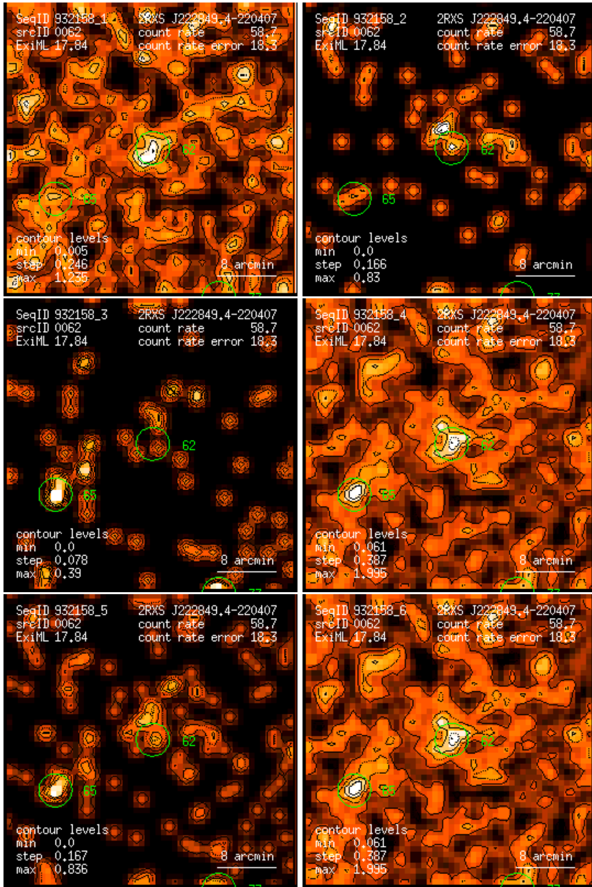
Figure 62: RASS 932158: detection 0062: band rate images, Gaussian filter: (1) PSPC channels 11 – 41, (2) 52 – 90, (3) 91 – 201, (4) 11 – 235, (5) 52 – 201, (6) 11 – 201. Broad band rates in counts/ks. Band rate contour levels in counts/ks/arcmin 2 .
