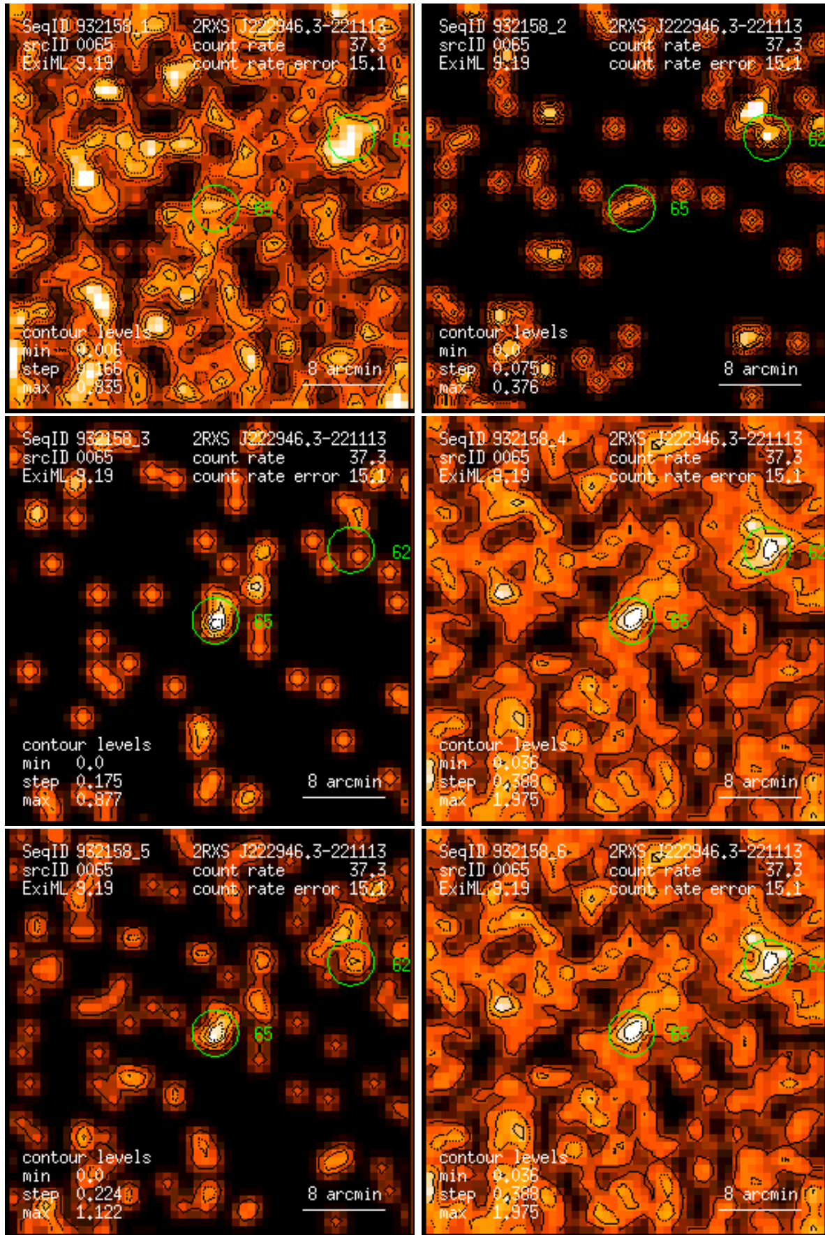
Figure 65: RASS 932158: detection 0065: band rate images, Gaussian filter: (1) PSPC channels 11 – 41, (2) 52 – 90, (3) 91 – 201, (4) 11 – 235, (5) 52 – 201, (6) 11 – 201. Broad band rates in counts/ks. Band rate contour levels in counts/ks/arcmin 2 .
