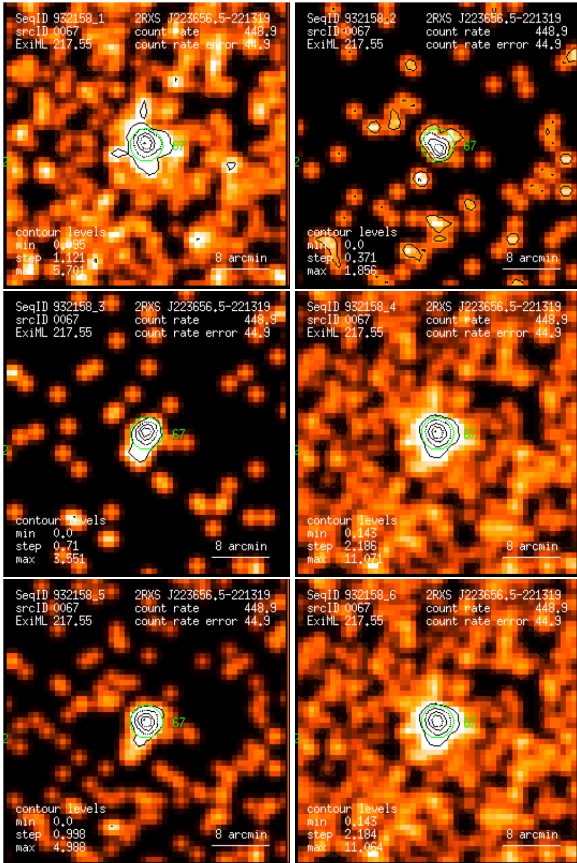
Figure 67: RASS 932158: detection 0067: band rate images, Gaussian filter: (1) PSPC channels 11 – 41, (2) 52 – 90, (3) 91 – 201, (4) 11 – 235, (5) 52 – 201, (6) 11 – 201. Broad band rates in counts/ks. Band rate contour levels in counts/ks/arcmin 2 .
