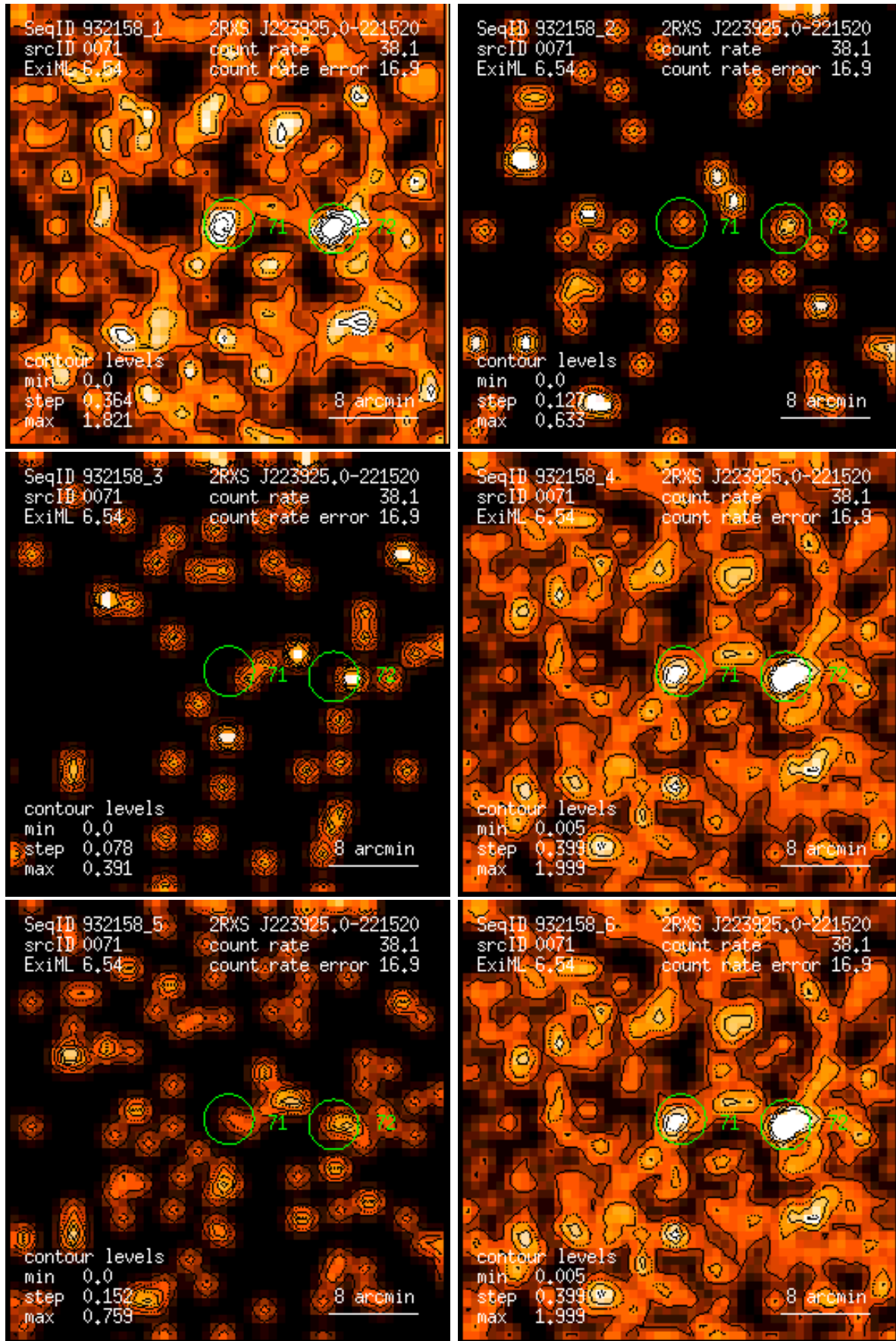
Figure 71: RASS 932158: detection 0071: band rate images, Gaussian filter: (1) PSPC channels 11 – 41, (2) 52 – 90, (3) 91 – 201, (4) 11 – 235, (5) 52 – 201, (6) 11 – 201. Broad band rates in counts/ks. Band rate contour levels in counts/ks/arcmin 2 .
