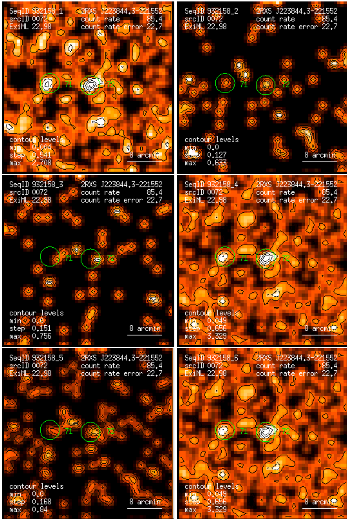
Figure 72: RASS 932158: detection 0072: band rate images, Gaussian filter: (1) PSPC channels 11 – 41, (2) 52 – 90, (3) 91 – 201, (4) 11 – 235, (5) 52 – 201, (6) 11 – 201. Broad band rates in counts/ks. Band rate contour levels in counts/ks/arcmin 2 .
