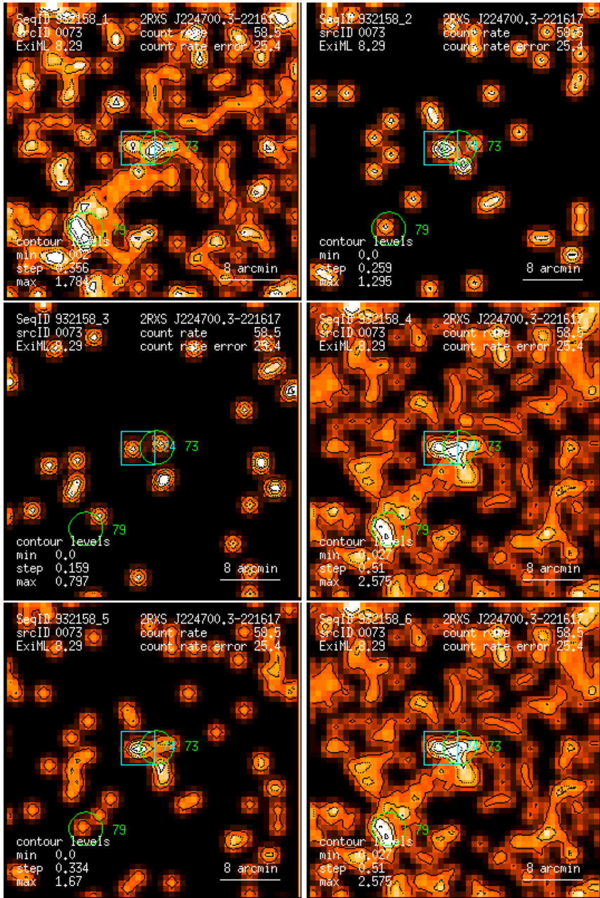
Figure 73: RASS 932158: detection 0073: band rate images, Gaussian filter: (1) PSPC channels 11 – 41, (2) 52 – 90, (3) 91 – 201, (4) 11 – 235, (5) 52 – 201, (6) 11 – 201. Broad band rates in counts/ks. Band rate contour levels in counts/ks/arcmin 2 .
