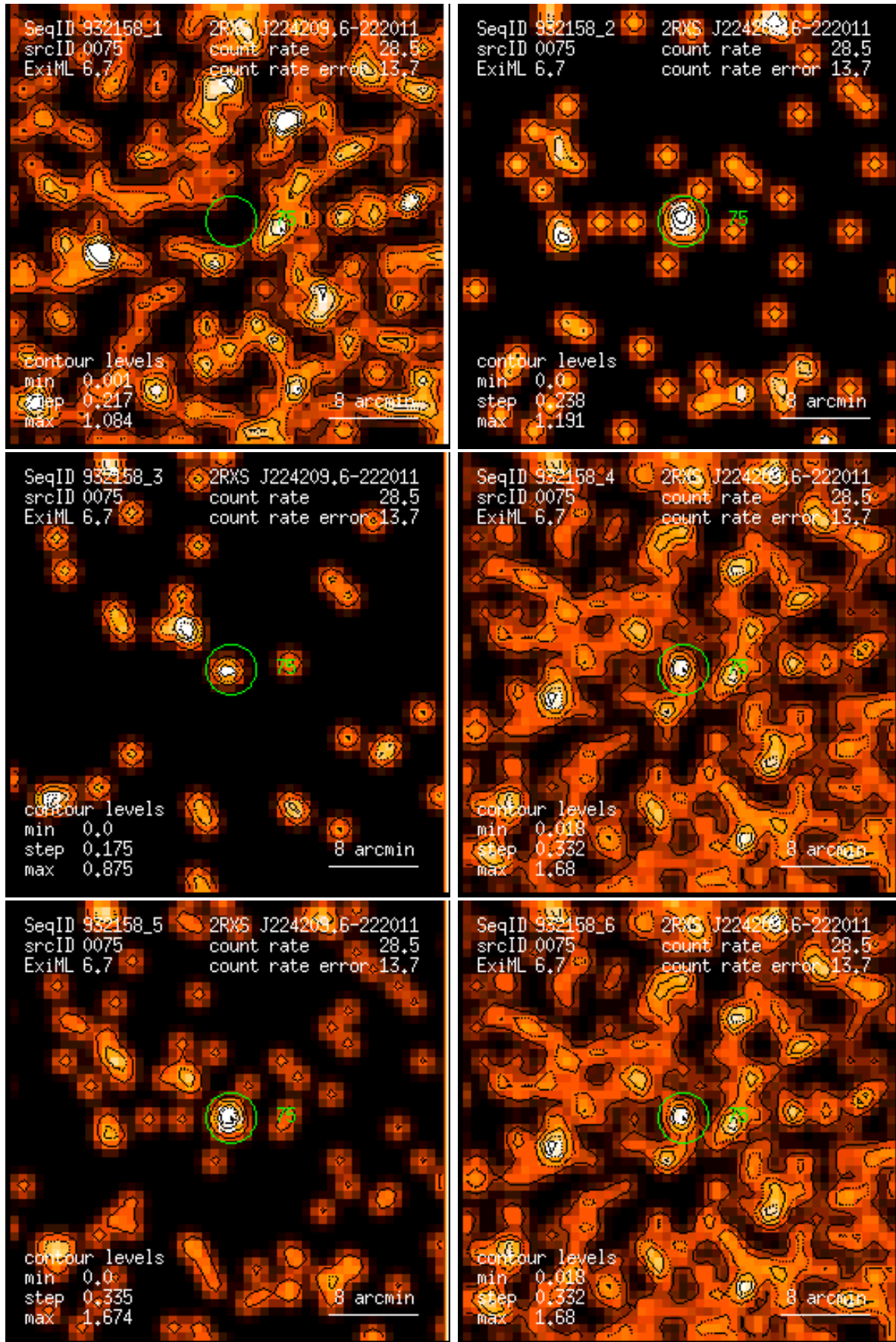
Figure 75: RASS 932158: detection 0075: band rate images, Gaussian filter: (1) PSPC channels 11 – 41, (2) 52 – 90, (3) 91 – 201, (4) 11 – 235, (5) 52 – 201, (6) 11 – 201. Broad band rates in counts/ks. Band rate contour levels in counts/ks/arcmin 2 .
