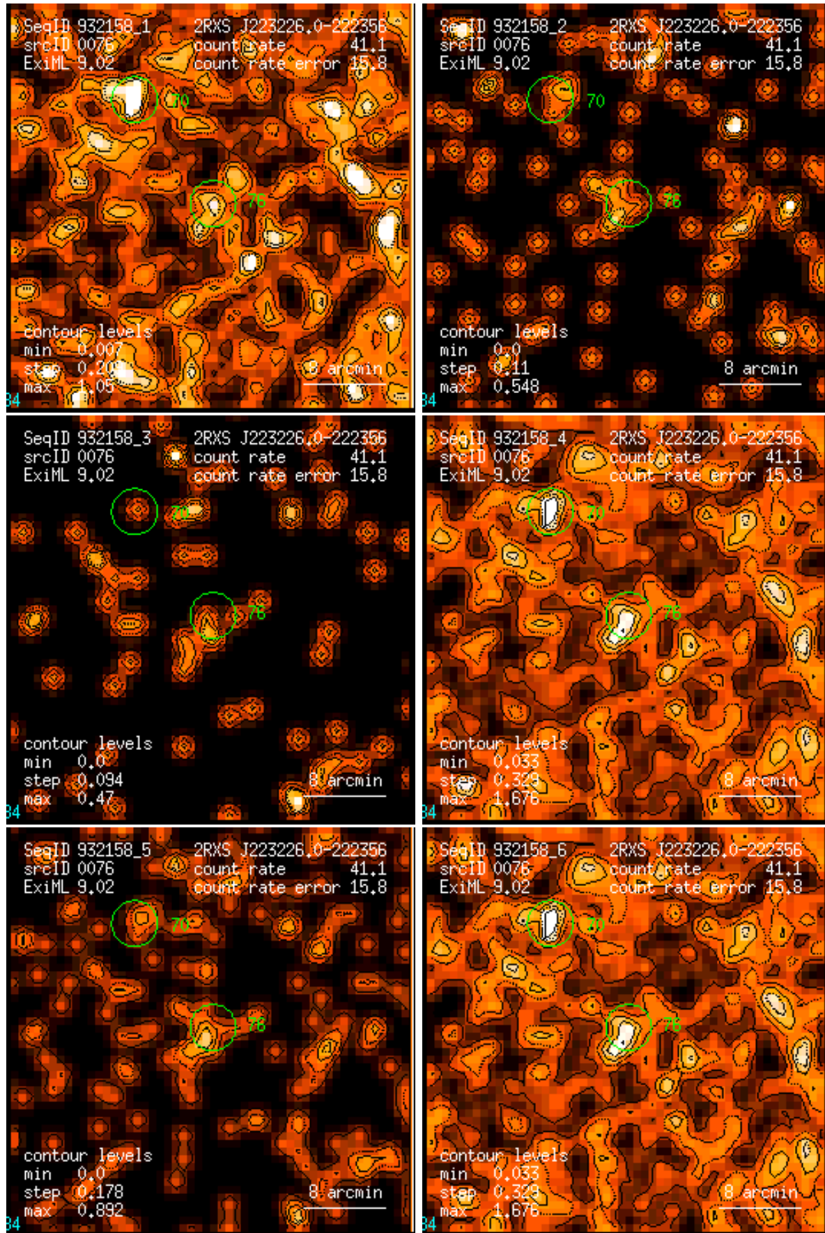
Figure 76: RASS 932158: detection 0076: band rate images, Gaussian filter: (1) PSPC channels 11 – 41, (2) 52 – 90, (3) 91 – 201, (4) 11 – 235, (5) 52 – 201, (6) 11 – 201. Broad band rates in counts/ks. Band rate contour levels in counts/ks/arcmin 2 .
