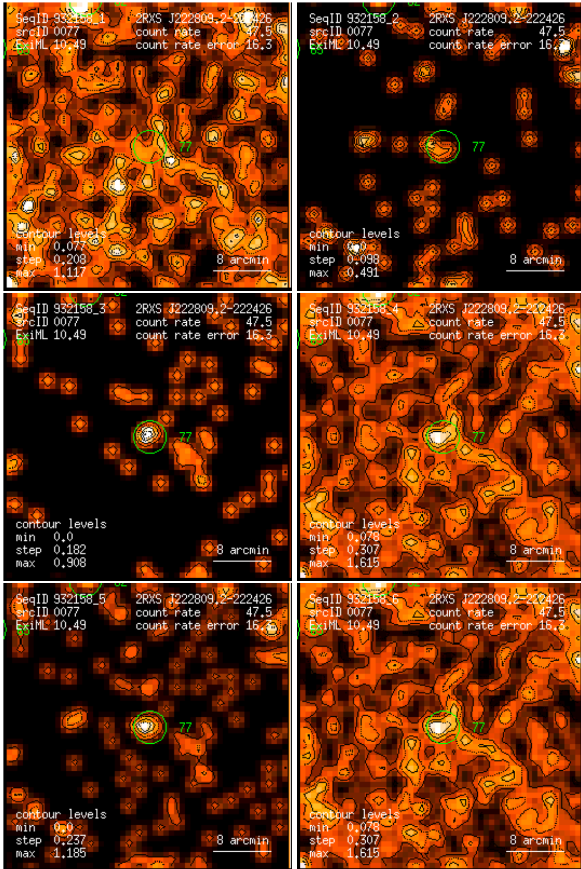
Figure 77: RASS 932158: detection 0077: band rate images, Gaussian filter: (1) PSPC channels 11 – 41, (2) 52 – 90, (3) 91 – 201, (4) 11 – 235, (5) 52 – 201, (6) 11 – 201. Broad band rates in counts/ks. Band rate contour levels in counts/ks/arcmin 2 .
