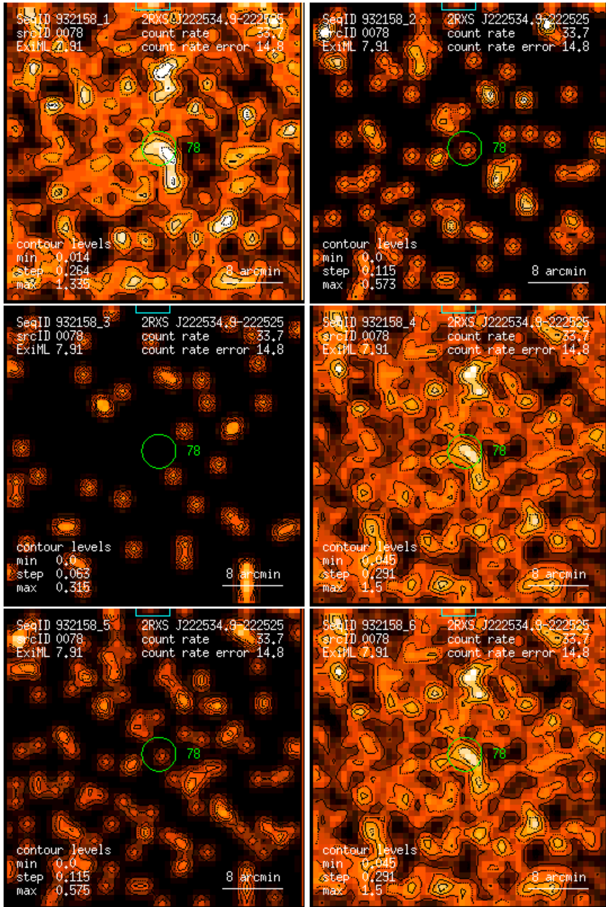
Figure 78: RASS 932158: detection 0078: band rate images, Gaussian filter: (1) PSPC channels 11 – 41, (2) 52 – 90, (3) 91 – 201, (4) 11 – 235, (5) 52 – 201, (6) 11 – 201. Broad band rates in counts/ks. Band rate contour levels in counts/ks/arcmin 2 .
