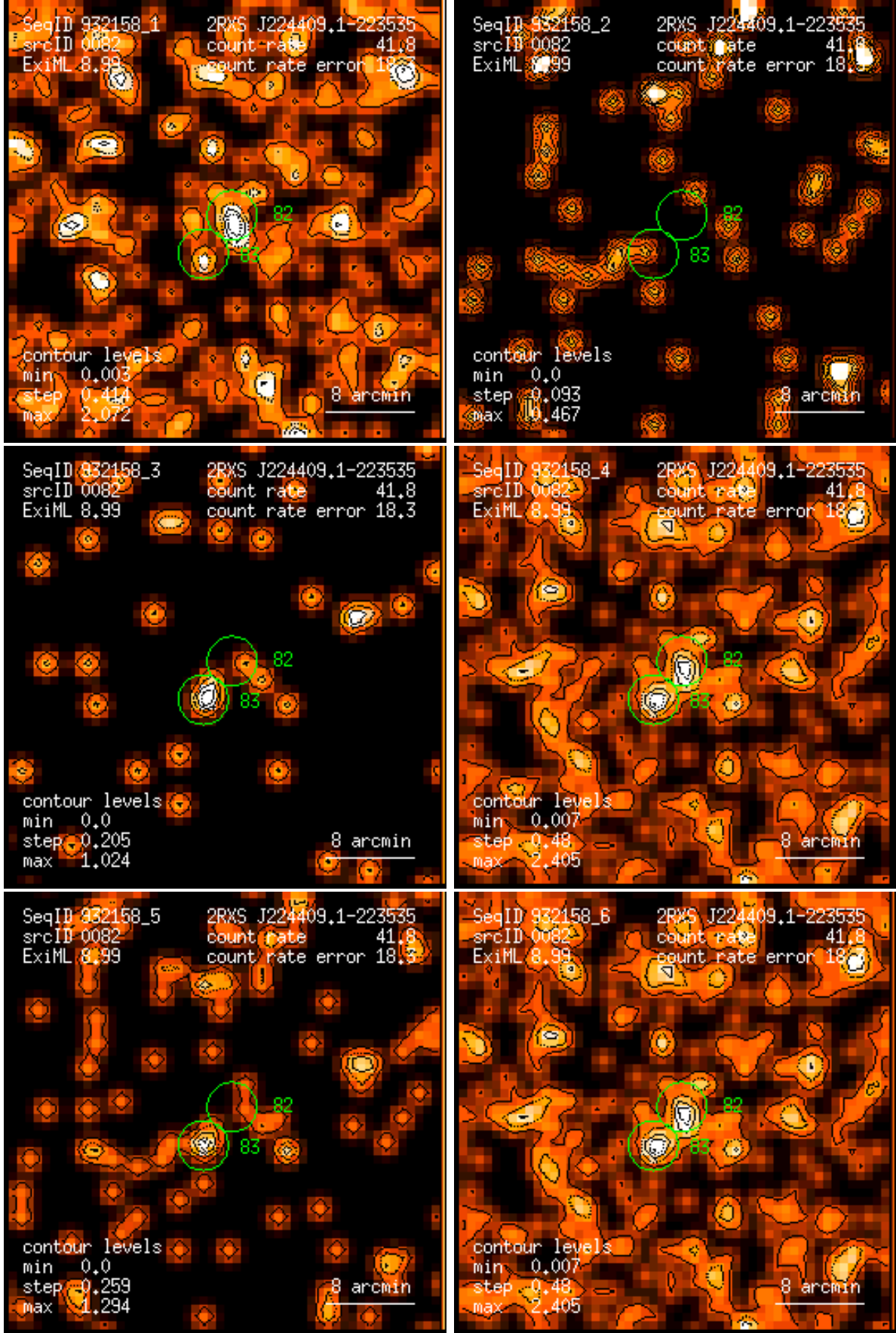
Figure 82: RASS 932158: detection 0082: band rate images, Gaussian filter: (1) PSPC channels 11 – 41, (2) 52 – 90, (3) 91 – 201, (4) 11 – 235, (5) 52 – 201, (6) 11 – 201. Broad band rates in counts/ks. Band rate contour levels in counts/ks/arcmin 2 .
