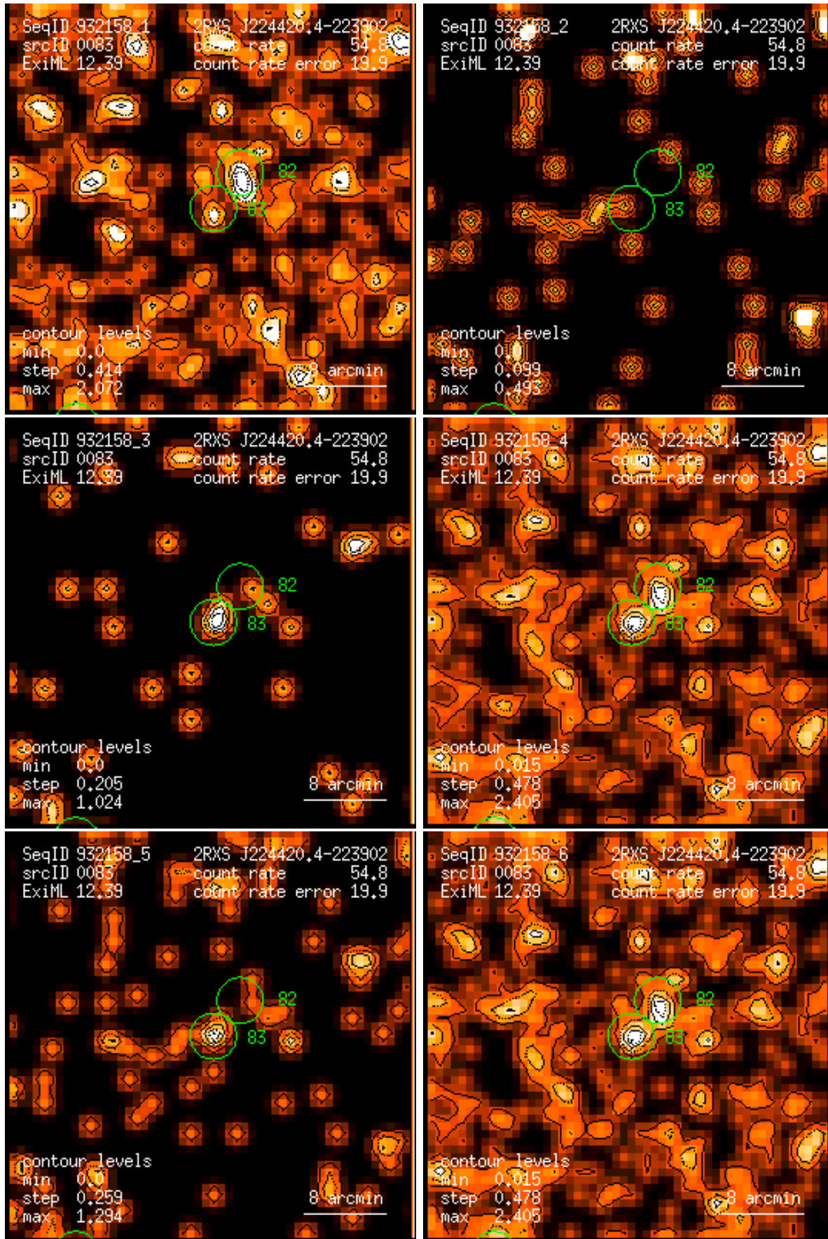
Figure 83: RASS 932158: detection 0083: band rate images, Gaussian filter: (1) PSPC channels 11 – 41, (2) 52 – 90, (3) 91 – 201, (4) 11 – 235, (5) 52 – 201, (6) 11 – 201. Broad band rates in counts/ks. Band rate contour levels in counts/ks/arcmin 2 .
