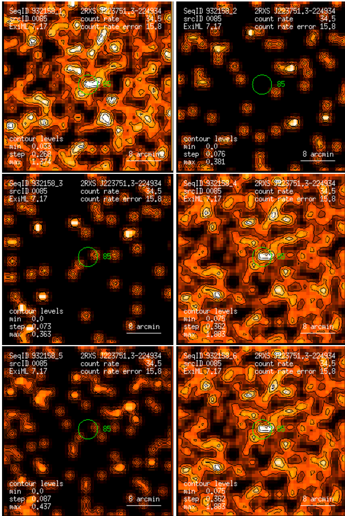
Figure 85: RASS 932158: detection 0085: band rate images, Gaussian filter: (1) PSPC channels 11 – 41, (2) 52 – 90, (3) 91 – 201, (4) 11 – 235, (5) 52 – 201, (6) 11 – 201. Broad band rates in counts/ks. Band rate contour levels in counts/ks/arcmin 2 .
