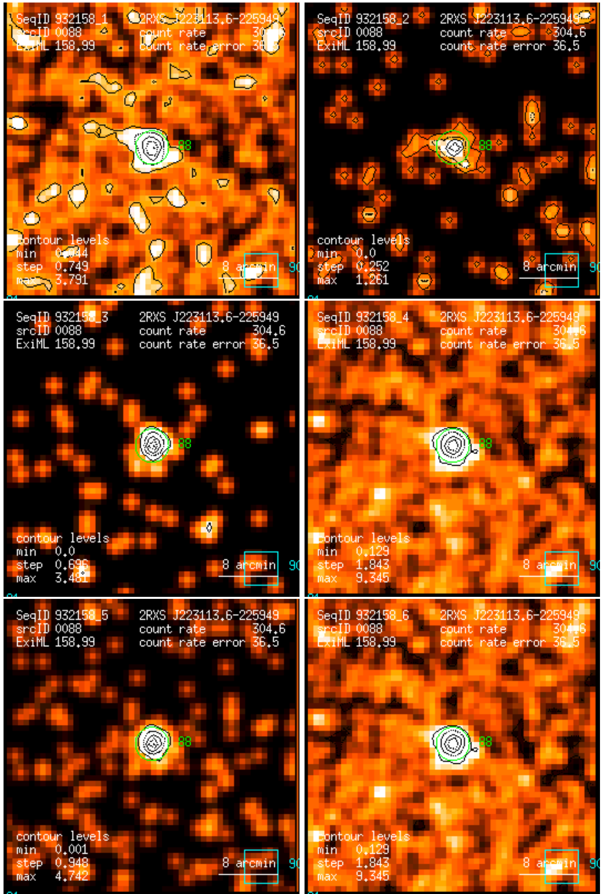
Figure 88: RASS 932158: detection 0088: band rate images, Gaussian filter: (1) PSPC channels 11 – 41, (2) 52 – 90, (3) 91 – 201, (4) 11 – 235, (5) 52 – 201, (6) 11 – 201. Broad band rates in counts/ks. Band rate contour levels in counts/ks/arcmin 2 .
