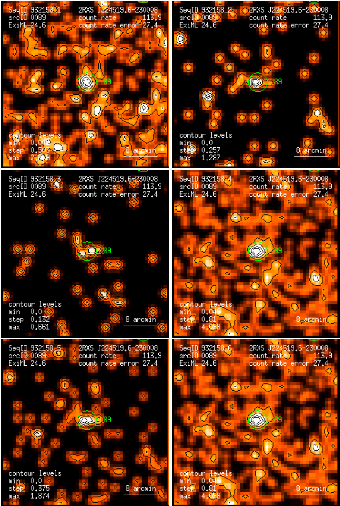
Figure 89: RASS 932158: detection 0089: band rate images, Gaussian filter: (1) PSPC channels 11 – 41, (2) 52 – 90, (3) 91 – 201, (4) 11 – 235, (5) 52 – 201, (6) 11 – 201. Broad band rates in counts/ks. Band rate contour levels in counts/ks/arcmin 2 .
