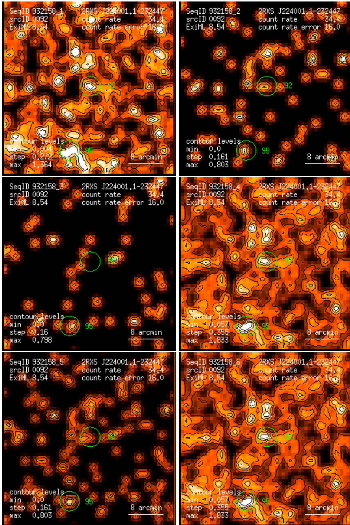
Figure 92: RASS 932158: detection 0092: band rate images, Gaussian filter: (1) PSPC channels 11 – 41, (2) 52 – 90, (3) 91 – 201, (4) 11 – 235, (5) 52 – 201, (6) 11 – 201. Broad band rates in counts/ks. Band rate contour levels in counts/ks/arcmin 2 .
