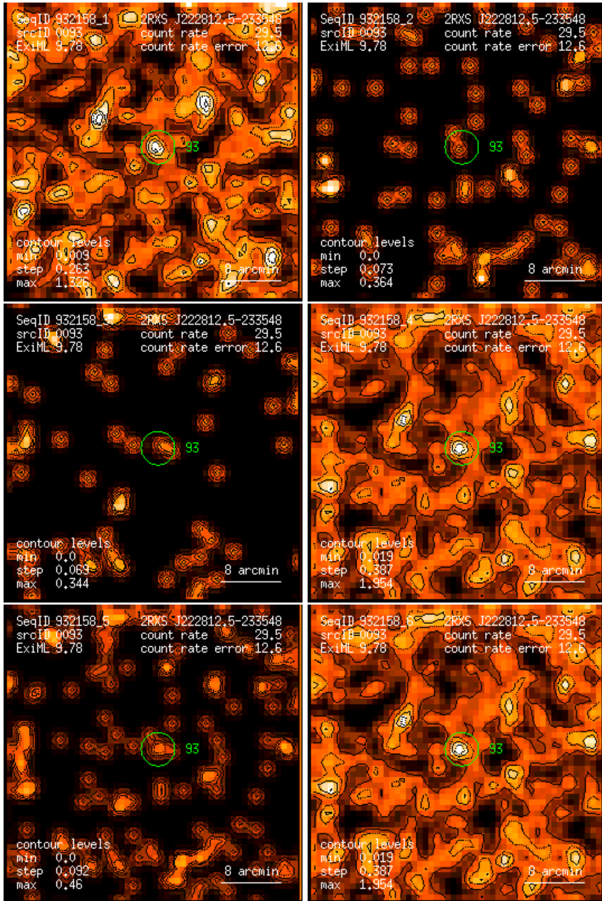
Figure 93: RASS 932158: detection 0093: band rate images, Gaussian filter: (1) PSPC channels 11 – 41, (2) 52 – 90, (3) 91 – 201, (4) 11 – 235, (5) 52 – 201, (6) 11 – 201. Broad band rates in counts/ks. Band rate contour levels in counts/ks/arcmin 2 .
