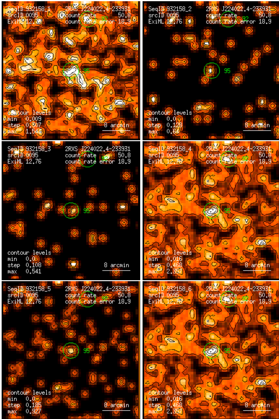
Figure 95: RASS 932158: detection 0095: band rate images, Gaussian filter: (1) PSPC channels 11 – 41, (2) 52 – 90, (3) 91 – 201, (4) 11 – 235, (5) 52 – 201, (6) 11 – 201. Broad band rates in counts/ks. Band rate contour levels in counts/ks/arcmin 2 .
