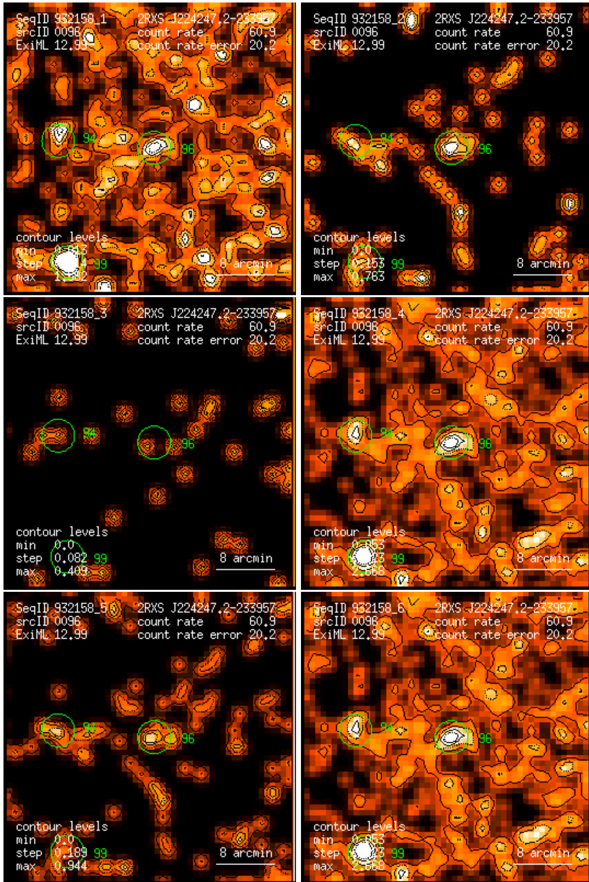
Figure 96: RASS 932158: detection 0096: band rate images, Gaussian filter: (1) PSPC channels 11 – 41, (2) 52 – 90, (3) 91 – 201, (4) 11 – 235, (5) 52 – 201, (6) 11 – 201. Broad band rates in counts/ks. Band rate contour levels in counts/ks/arcmin 2 .
