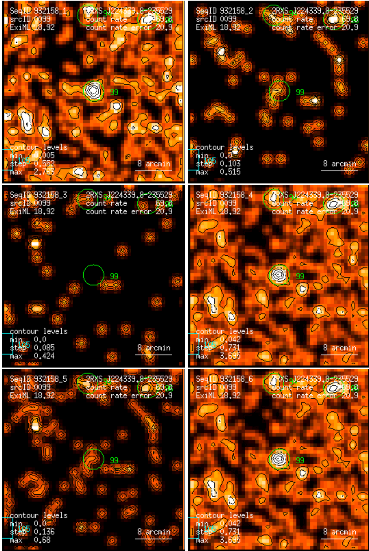
Figure 99: RASS 932158: detection 0099: band rate images, Gaussian filter: (1) PSPC channels 11 – 41, (2) 52 – 90, (3) 91 – 201, (4) 11 – 235, (5) 52 – 201, (6) 11 – 201. Broad band rates in counts/ks. Band rate contour levels in counts/ks/arcmin 2 .
