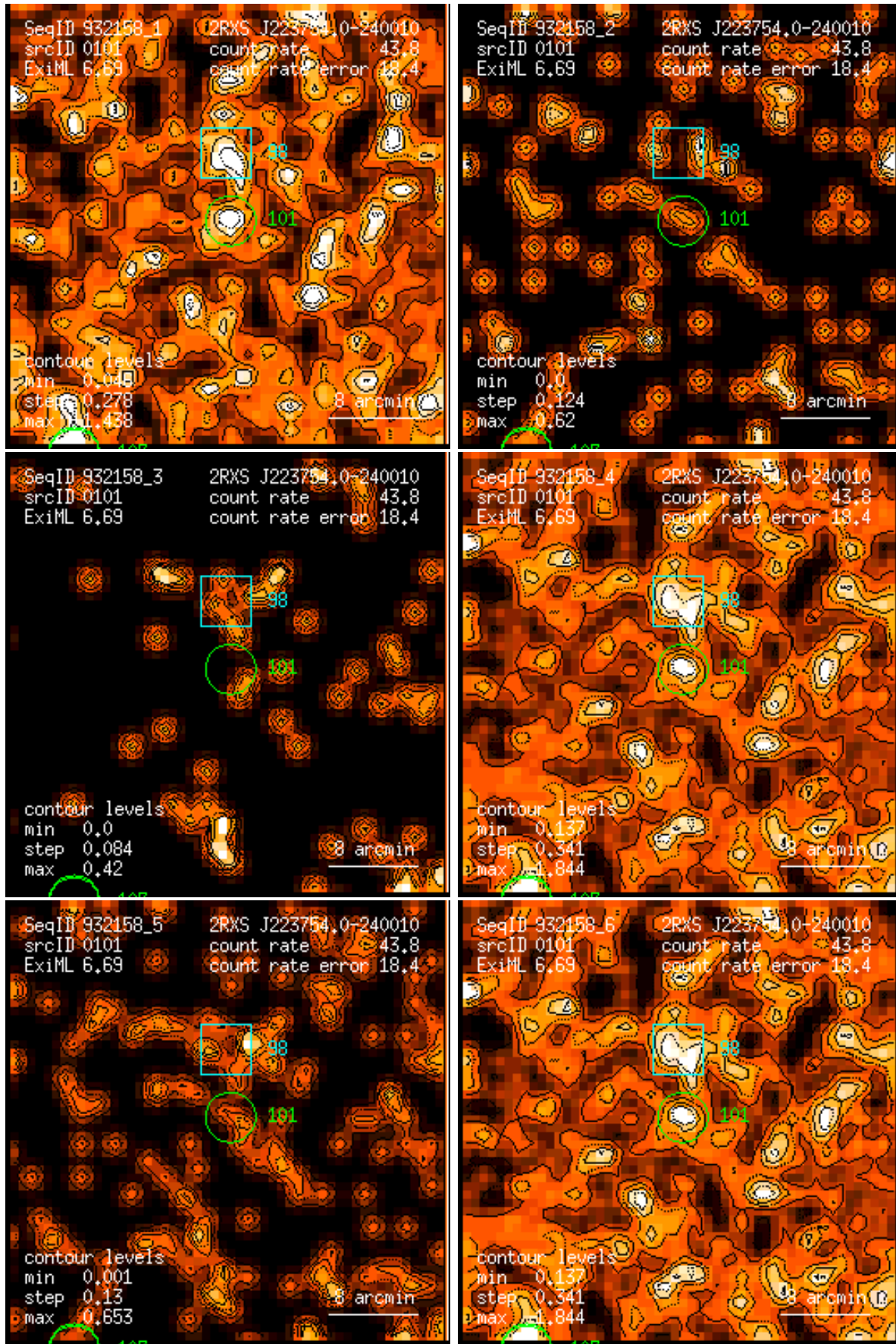
Figure 101: RASS 932158: detection 0101: band rate images, Gaussian filter: (1) PSPC channels 11 – 41, (2) 52 – 90, (3) 91 – 201, (4) 11 – 235, (5) 52 – 201, (6) 11 – 201. Broad band rates in counts/ks. Band rate contour levels in counts/ks/arcmin 2 .
