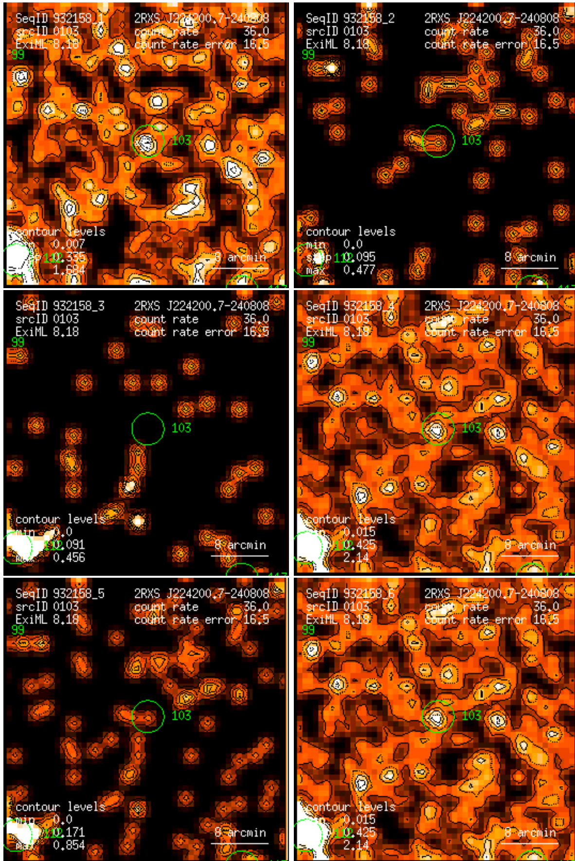
Figure 103: RASS 932158: detection 0103: band rate images, Gaussian filter: (1) PSPC channels 11 – 41, (2) 52 – 90, (3) 91 – 201, (4) 11 – 235, (5) 52 – 201, (6) 11 – 201. Broad band rates in counts/ks. Band rate contour levels in counts/ks/arcmin 2 .
