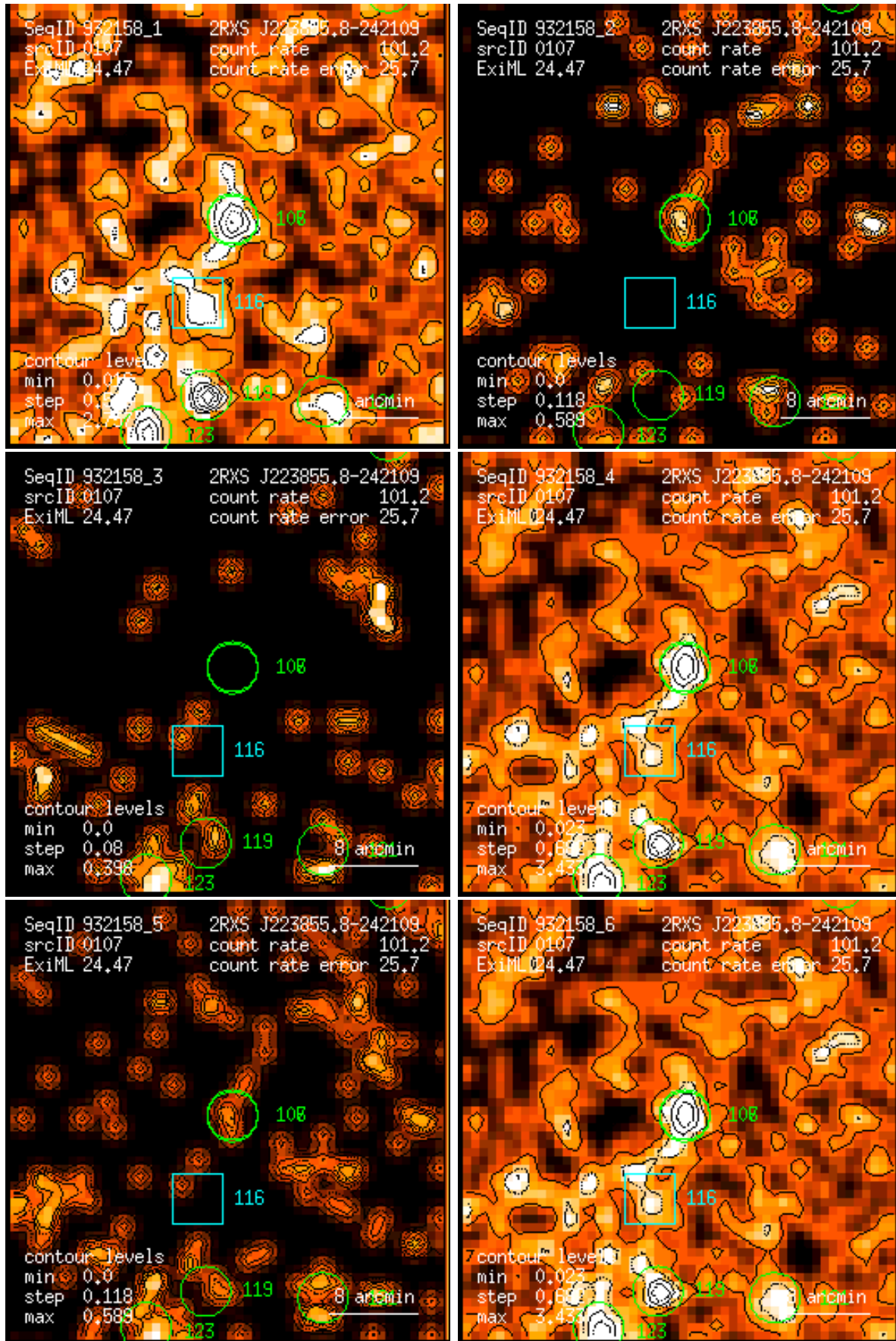
Figure 107: RASS 932158: detection 0107: band rate images, Gaussian filter: (1) PSPC channels 11 – 41, (2) 52 – 90, (3) 91 – 201, (4) 11 – 235, (5) 52 – 201, (6) 11 – 201. Broad band rates in counts/ks. Band rate contour levels in counts/ks/arcmin 2 .
