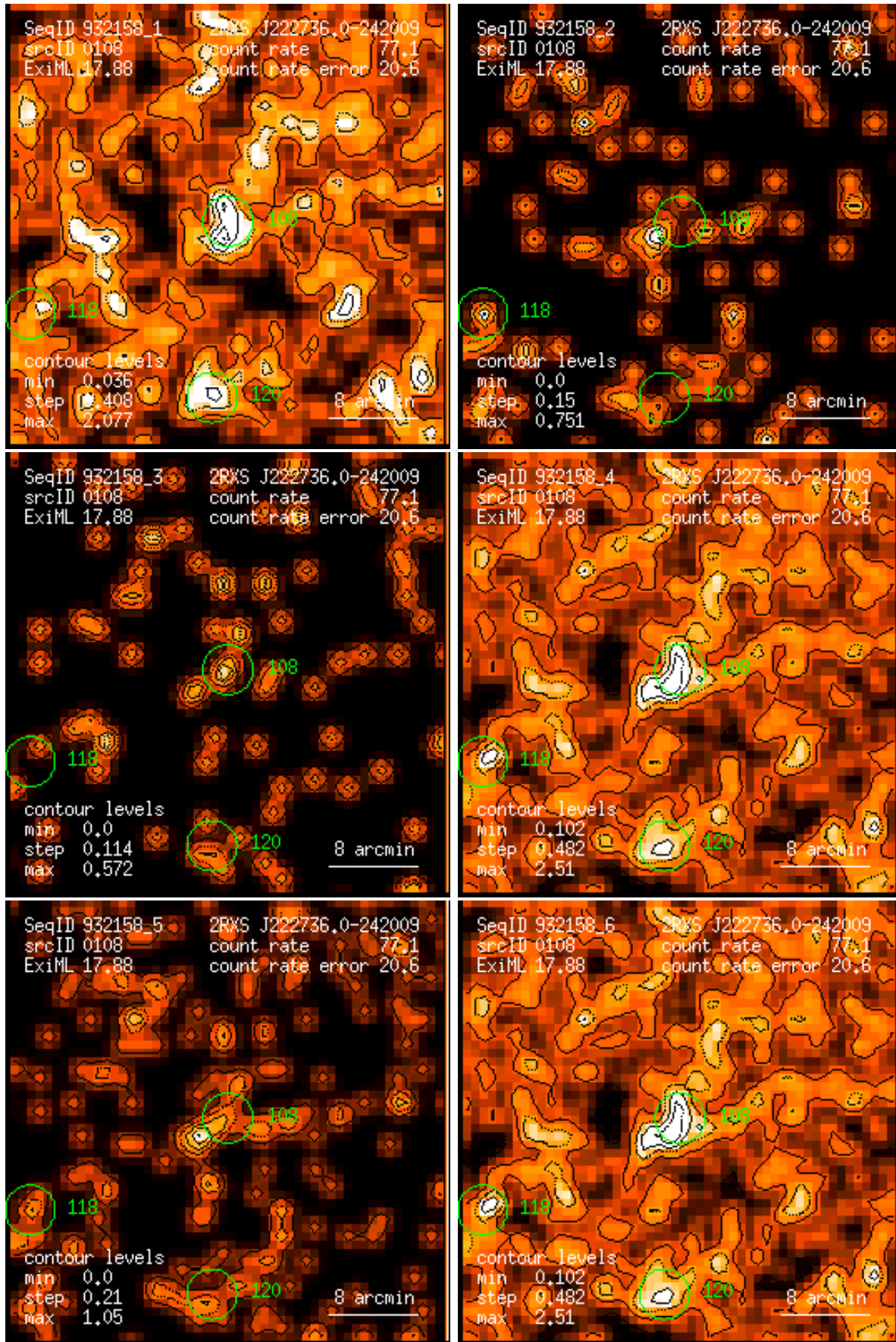
Figure 108: RASS 932158: detection 0108: band rate images, Gaussian filter: (1) PSPC channels 11 – 41, (2) 52 – 90, (3) 91 – 201, (4) 11 – 235, (5) 52 – 201, (6) 11 – 201. Broad band rates in counts/ks. Band rate contour levels in counts/ks/arcmin 2 .
