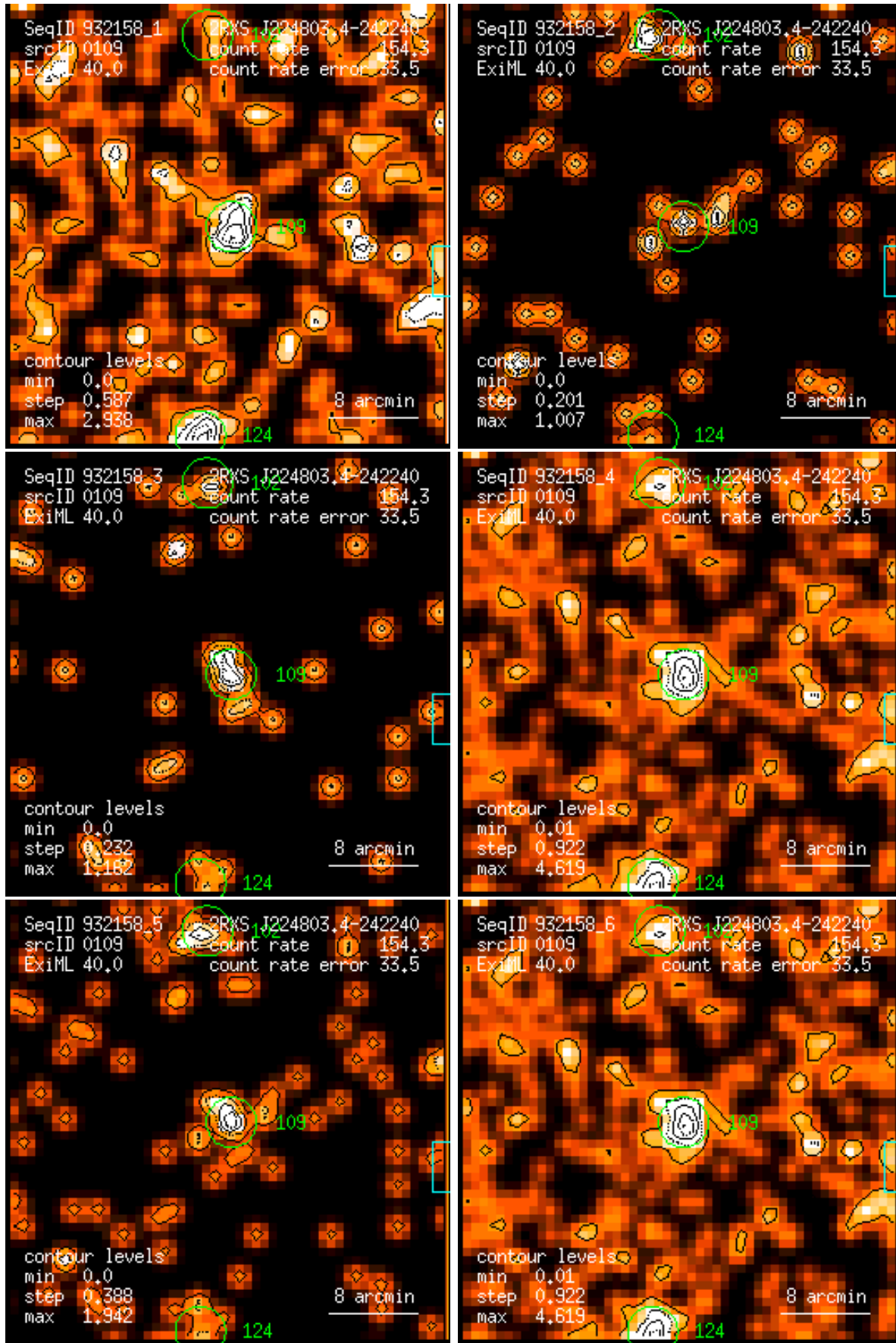
Figure 109: RASS 932158: detection 0109: band rate images, Gaussian filter: (1) PSPC channels 11 – 41, (2) 52 – 90, (3) 91 – 201, (4) 11 – 235, (5) 52 – 201, (6) 11 – 201. Broad band rates in counts/ks. Band rate contour levels in counts/ks/arcmin 2 .
