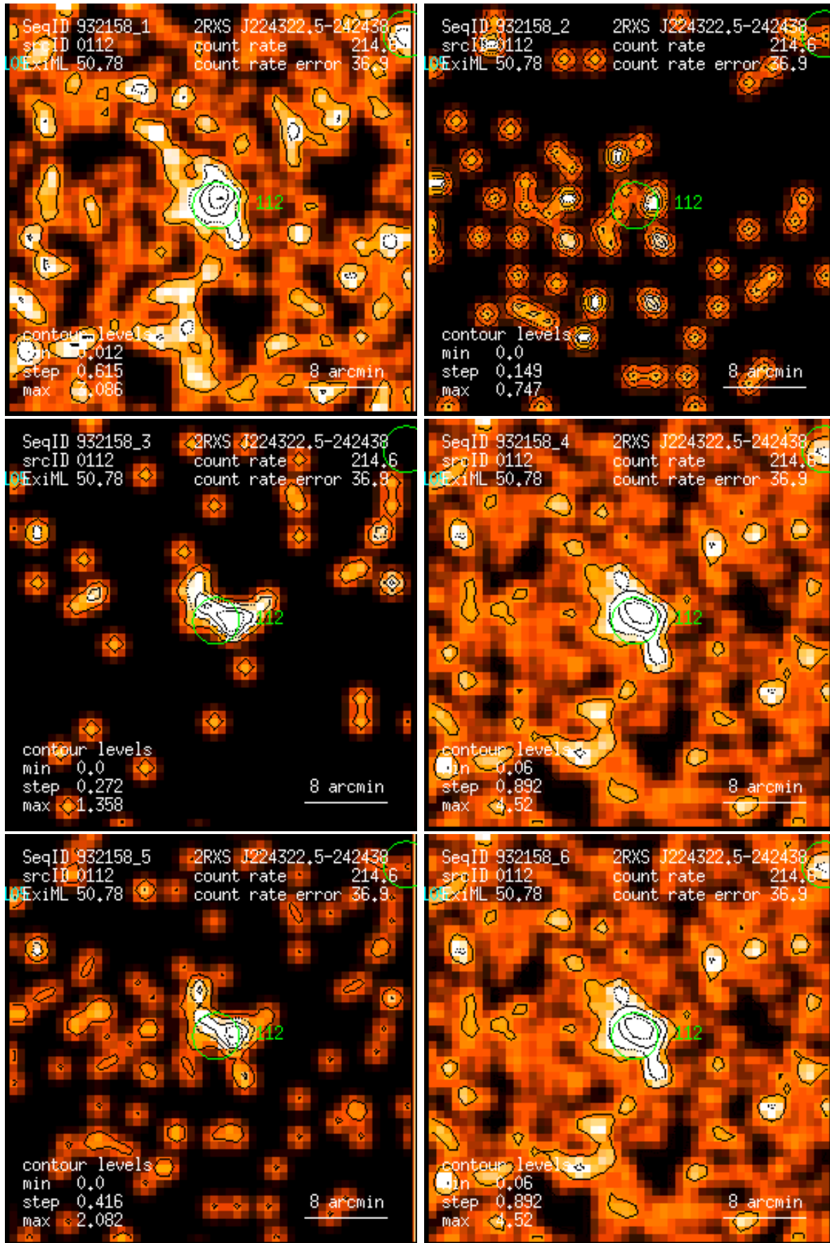
Figure 112: RASS 932158: detection 0112: band rate images, Gaussian filter: (1) PSPC channels 11 – 41, (2) 52 – 90, (3) 91 – 201, (4) 11 – 235, (5) 52 – 201, (6) 11 – 201. Broad band rates in counts/ks. Band rate contour levels in counts/ks/arcmin 2 .
