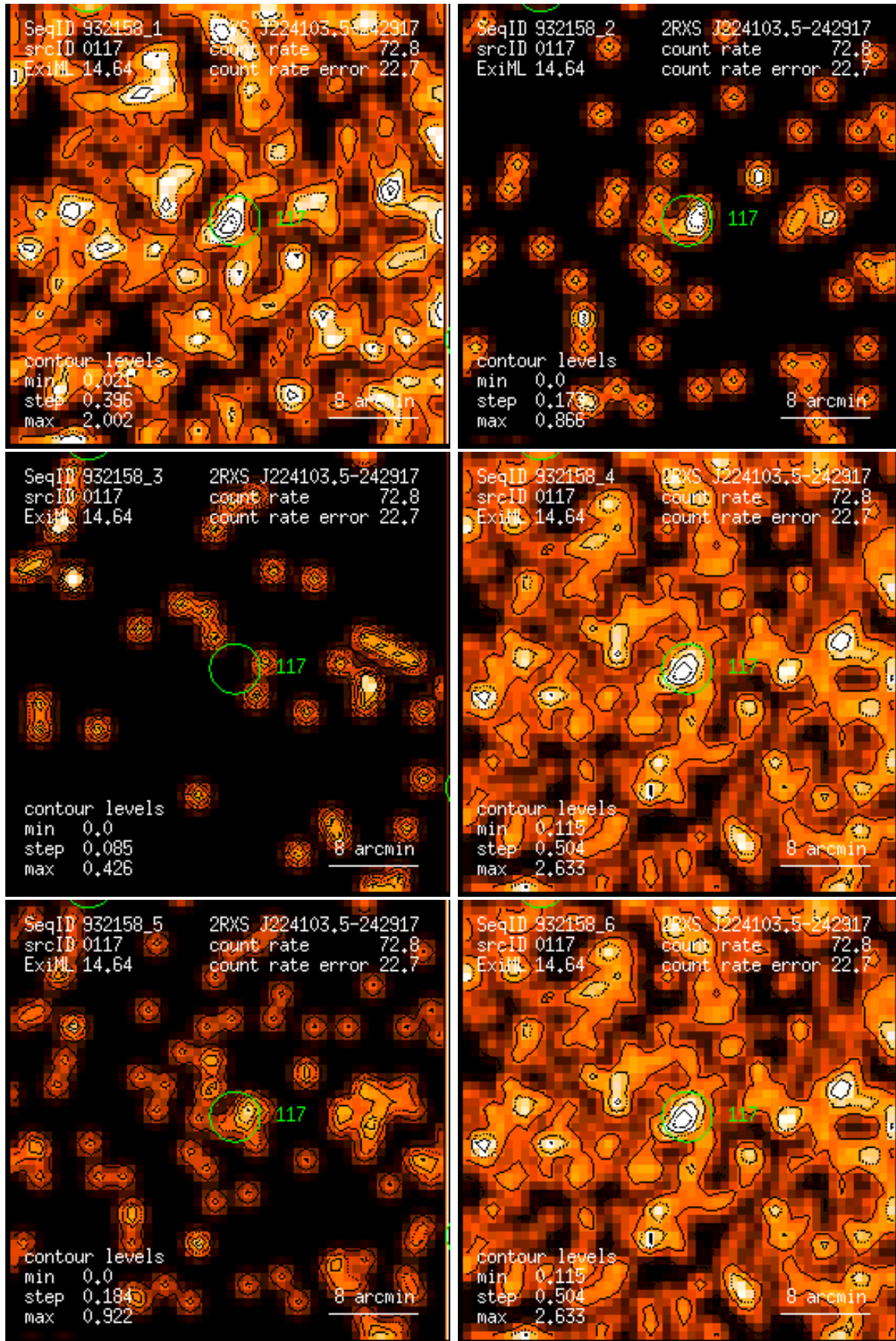
Figure 117: RASS 932158: detection 0117: band rate images, Gaussian filter: (1) PSPC channels 11 – 41, (2) 52 – 90, (3) 91 – 201, (4) 11 – 235, (5) 52 – 201, (6) 11 – 201. Broad band rates in counts/ks. Band rate contour levels in counts/ks/arcmin 2 .
