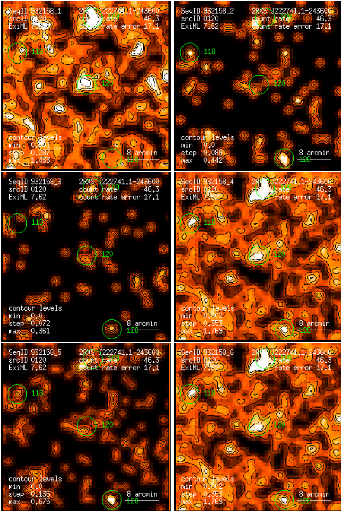
Figure 120: RASS 932158: detection 0120: band rate images, Gaussian filter: (1) PSPC channels 11 – 41, (2) 52 – 90, (3) 91 – 201, (4) 11 – 235, (5) 52 – 201, (6) 11 – 201. Broad band rates in counts/ks. Band rate contour levels in counts/ks/arcmin 2 .
