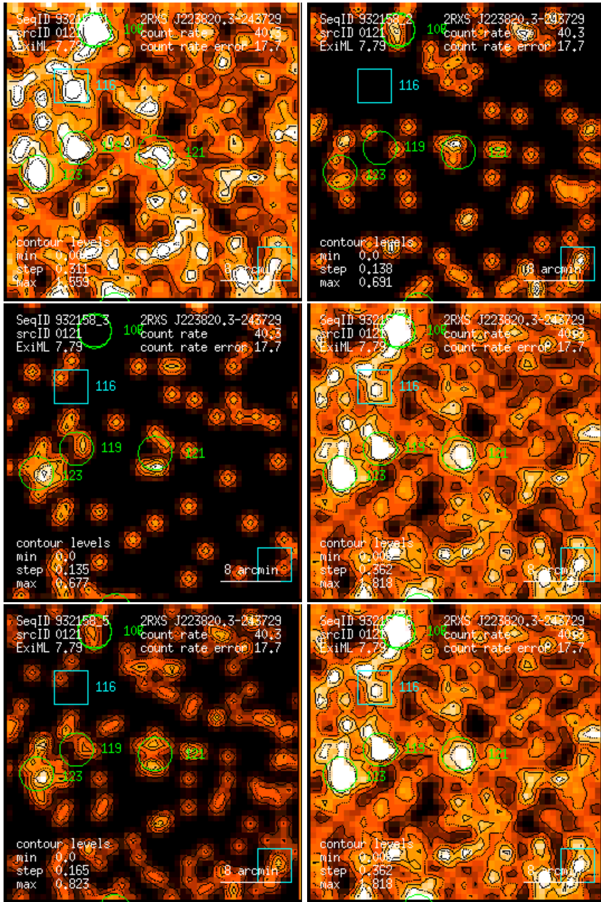
Figure 121: RASS 932158: detection 0121: band rate images, Gaussian filter: (1) PSPC channels 11 – 41, (2) 52 – 90, (3) 91 – 201, (4) 11 – 235, (5) 52 – 201, (6) 11 – 201. Broad band rates in counts/ks. Band rate contour levels in counts/ks/arcmin 2 .
