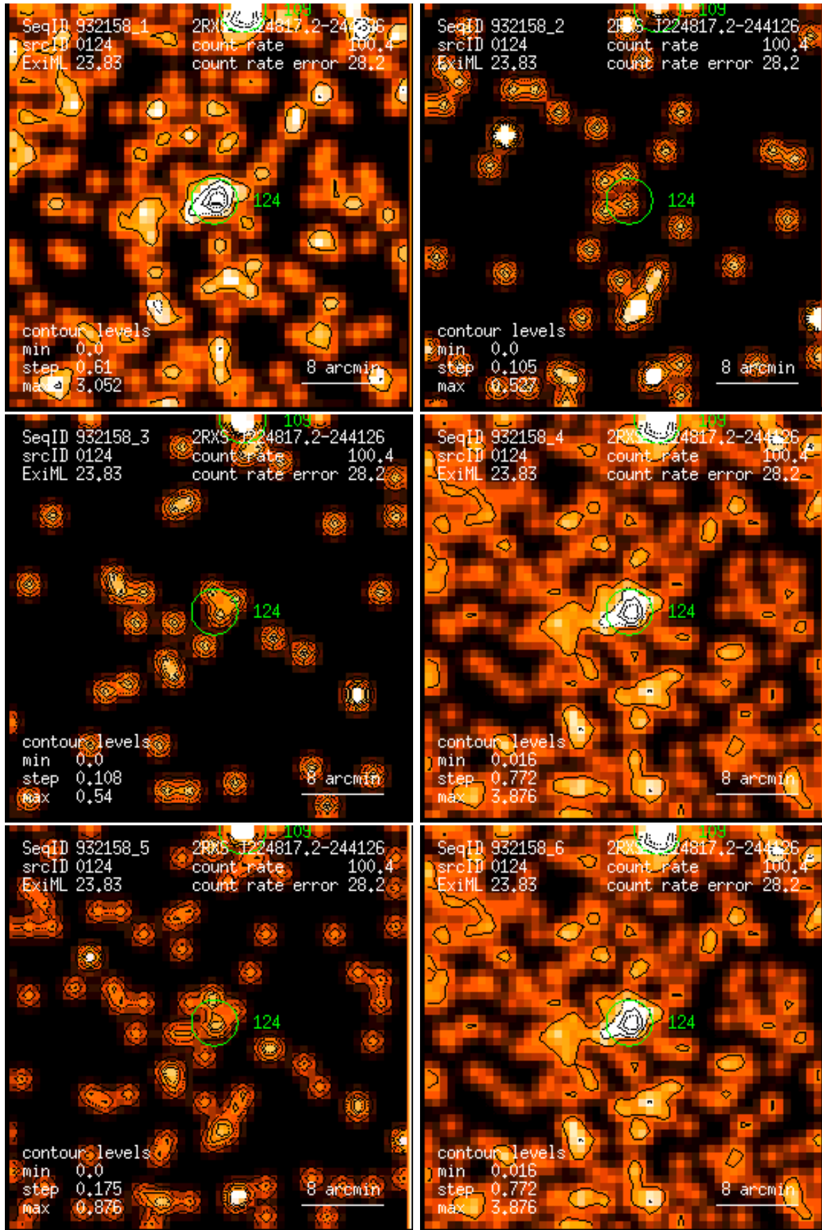
Figure 124: RASS 932158: detection 0124: band rate images, Gaussian filter: (1) PSPC channels 11 – 41, (2) 52 – 90, (3) 91 – 201, (4) 11 – 235, (5) 52 – 201, (6) 11 – 201. Broad band rates in counts/ks. Band rate contour levels in counts/ks/arcmin 2 .
